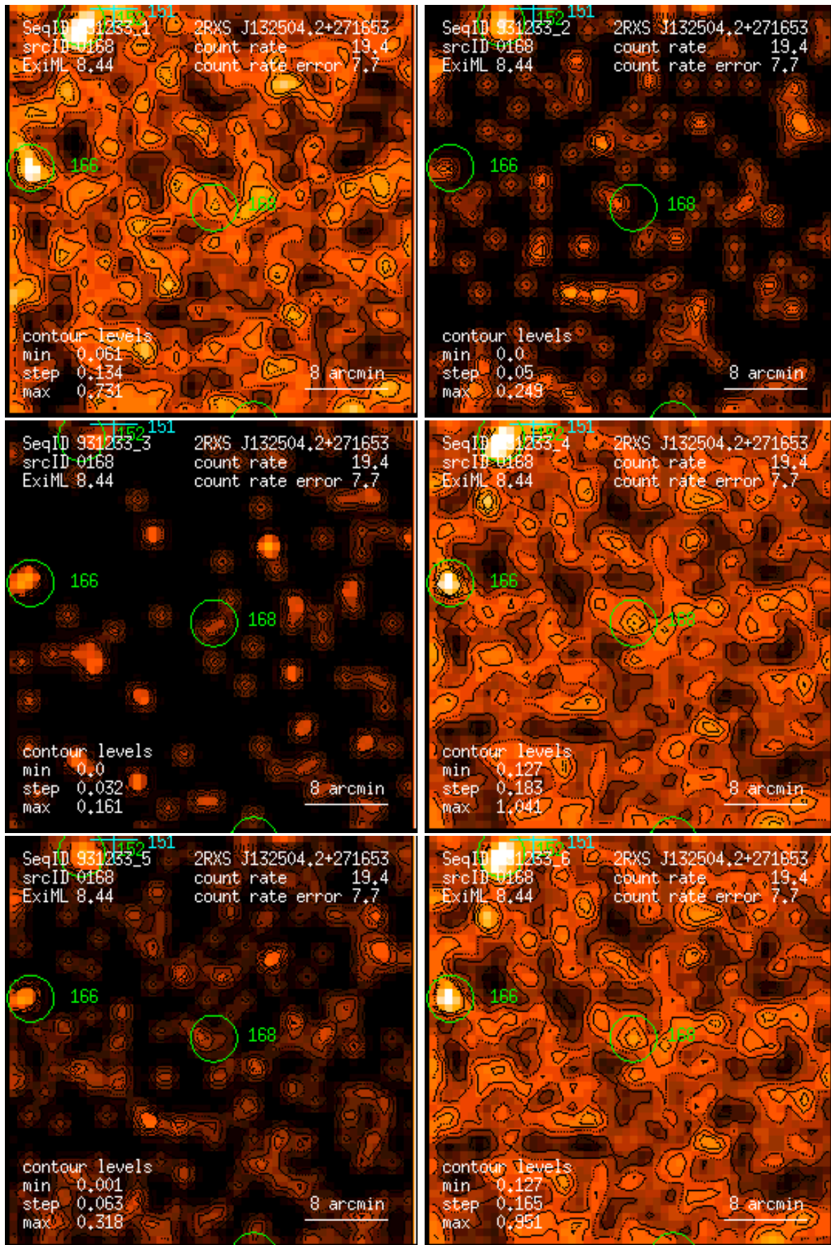
Figure 168: RASS 931233: detection 0168: band rate images, Gaussian filter: (1) PSPC channels 11 – 41, (2) 52 – 90, (3) 91 – 201, (4) 11 – 235, (5) 52 – 201, (6) 11 – 201. Broad band rates in counts/ks. Band rate contour levels in counts/ks/arcmin 2 .
