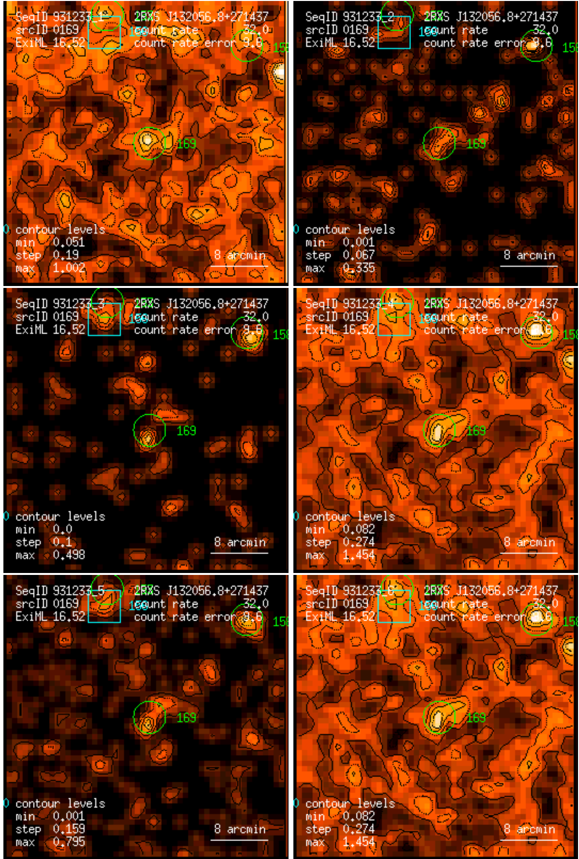
Figure 169: RASS 931233: detection 0169: band rate images, Gaussian filter: (1) PSPC channels 11 – 41, (2) 52 – 90, (3) 91 – 201, (4) 11 – 235, (5) 52 – 201, (6) 11 – 201. Broad band rates in counts/ks. Band rate contour levels in counts/ks/arcmin 2 .
