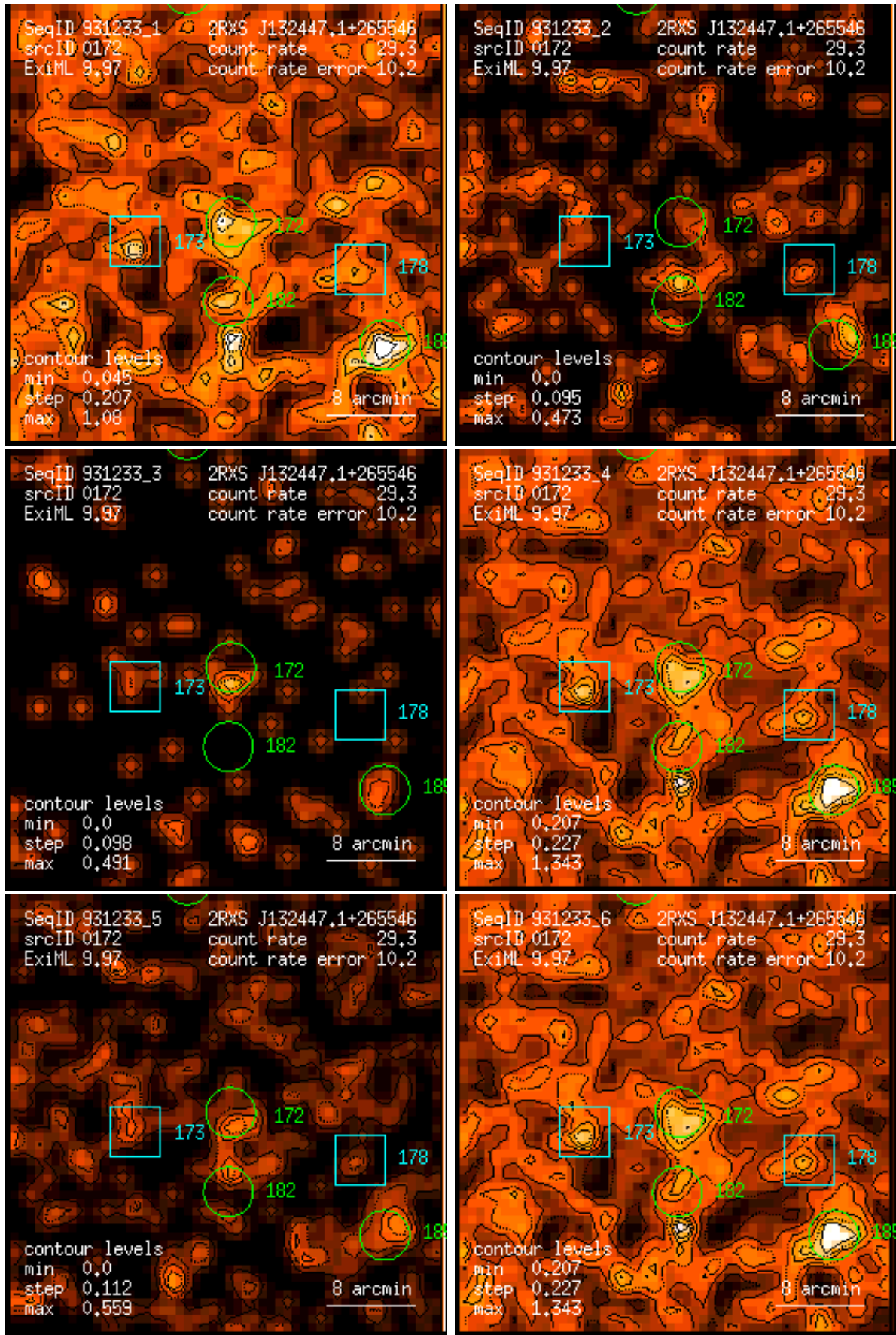
Figure 172: RASS 931233: detection 0172: band rate images, Gaussian filter: (1) PSPC channels 11 – 41, (2) 52 – 90, (3) 91 – 201, (4) 11 – 235, (5) 52 – 201, (6) 11 – 201. Broad band rates in counts/ks. Band rate contour levels in counts/ks/arcmin 2 .
