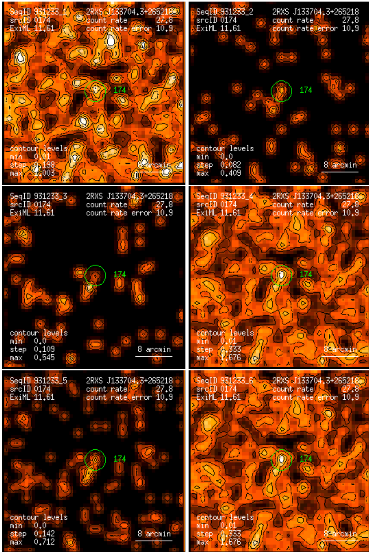
Figure 174: RASS 931233: detection 0174: band rate images, Gaussian filter: (1) PSPC channels 11 – 41, (2) 52 – 90, (3) 91 – 201, (4) 11 – 235, (5) 52 – 201, (6) 11 – 201. Broad band rates in counts/ks. Band rate contour levels in counts/ks/arcmin 2 .
