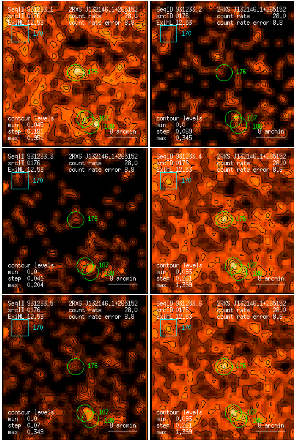
Figure 176: RASS 931233: detection 0176: band rate images, Gaussian filter: (1) PSPC channels 11 – 41, (2) 52 – 90, (3) 91 – 201, (4) 11 – 235, (5) 52 – 201, (6) 11 – 201. Broad band rates in counts/ks. Band rate contour levels in counts/ks/arcmin 2 .
