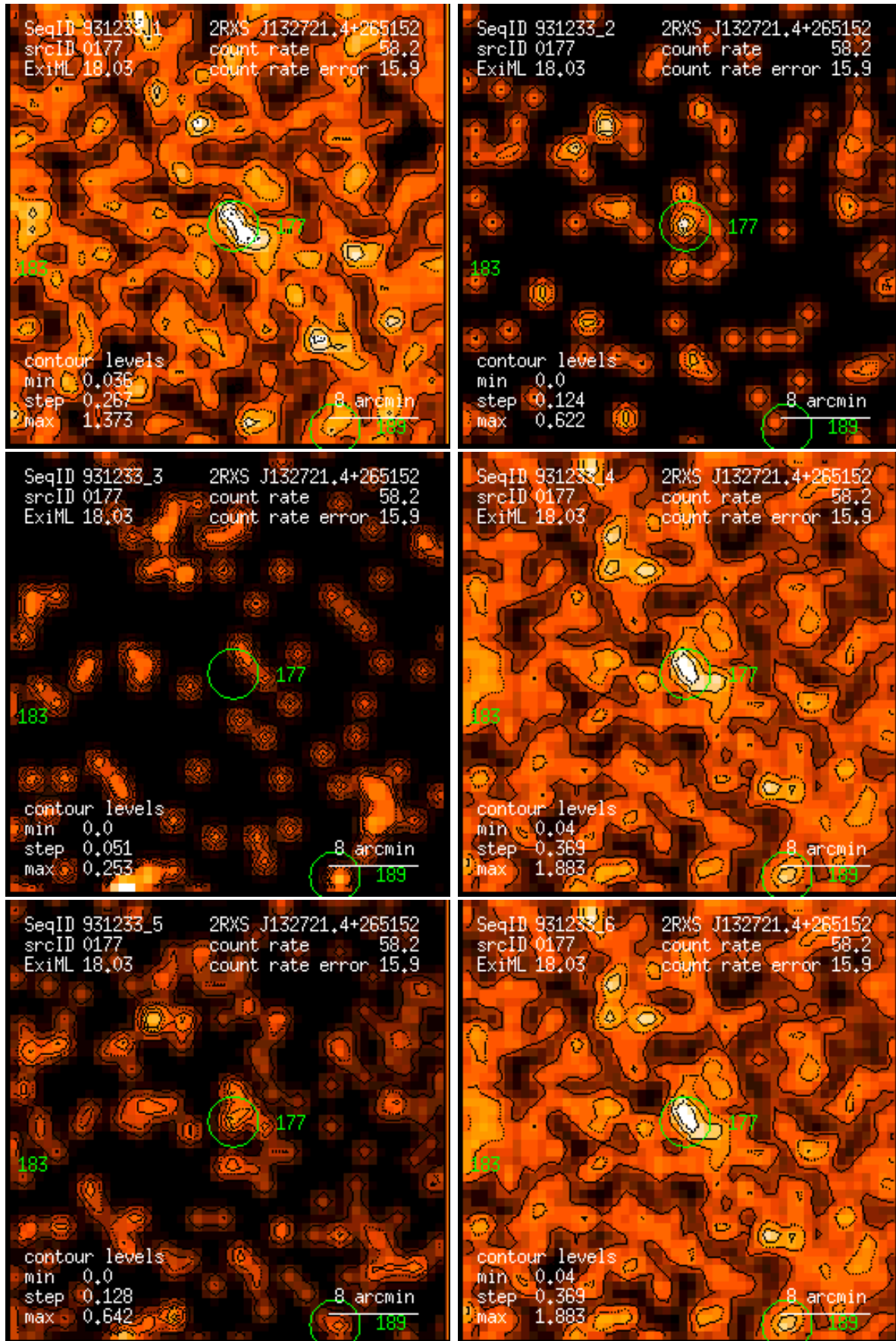
Figure 177: RASS 931233: detection 0177: band rate images, Gaussian filter: (1) PSPC channels 11 – 41, (2) 52 – 90, (3) 91 – 201, (4) 11 – 235, (5) 52 – 201, (6) 11 – 201. Broad band rates in counts/ks. Band rate contour levels in counts/ks/arcmin 2 .
