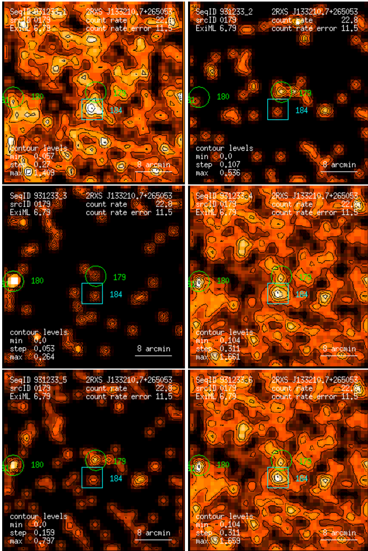
Figure 179: RASS 931233: detection 0179: band rate images, Gaussian filter: (1) PSPC channels 11 – 41, (2) 52 – 90, (3) 91 – 201, (4) 11 – 235, (5) 52 – 201, (6) 11 – 201. Broad band rates in counts/ks. Band rate contour levels in counts/ks/arcmin 2 .
