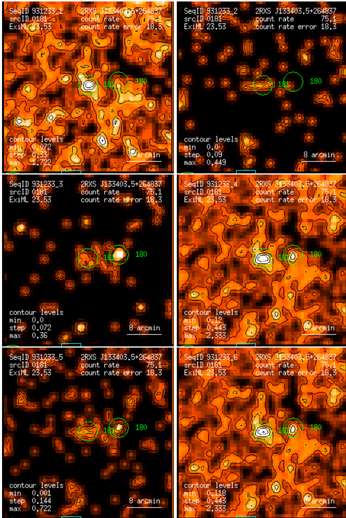
Figure 181: RASS 931233: detection 0181: band rate images, Gaussian filter: (1) PSPC channels 11 – 41, (2) 52 – 90, (3) 91 – 201, (4) 11 – 235, (5) 52 – 201, (6) 11 – 201. Broad band rates in counts/ks. Band rate contour levels in counts/ks/arcmin 2 .
