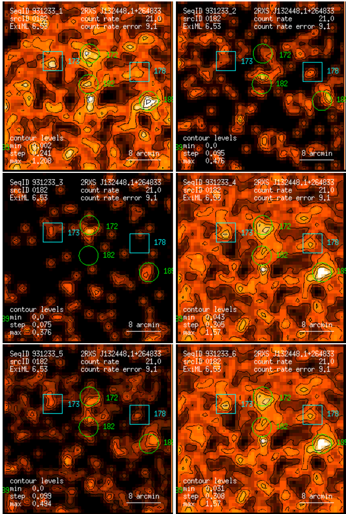
Figure 182: RASS 931233: detection 0182: band rate images, Gaussian filter: (1) PSPC channels 11 – 41, (2) 52 – 90, (3) 91 – 201, (4) 11 – 235, (5) 52 – 201, (6) 11 – 201. Broad band rates in counts/ks. Band rate contour levels in counts/ks/arcmin 2 .
