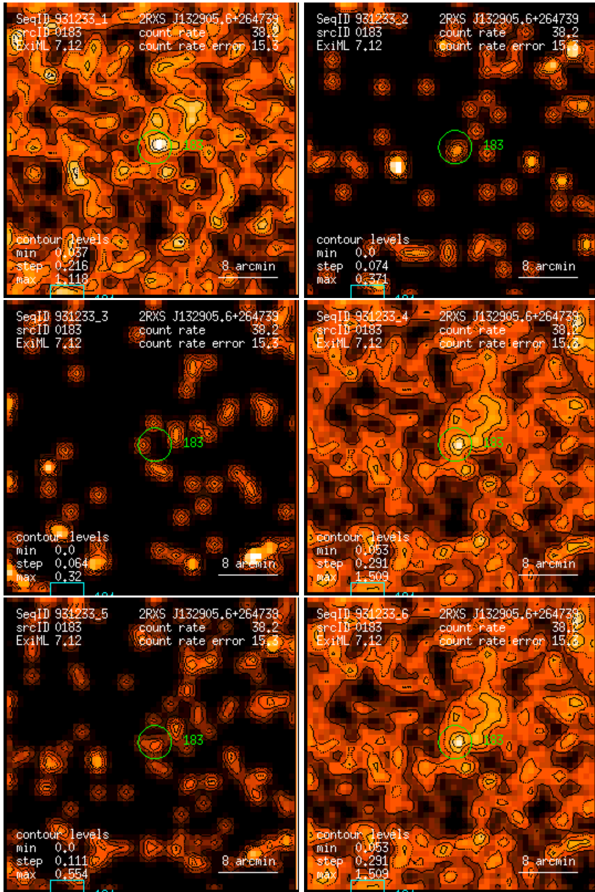
Figure 183: RASS 931233: detection 0183: band rate images, Gaussian filter: (1) PSPC channels 11 – 41, (2) 52 – 90, (3) 91 – 201, (4) 11 – 235, (5) 52 – 201, (6) 11 – 201. Broad band rates in counts/ks. Band rate contour levels in counts/ks/arcmin 2 .
