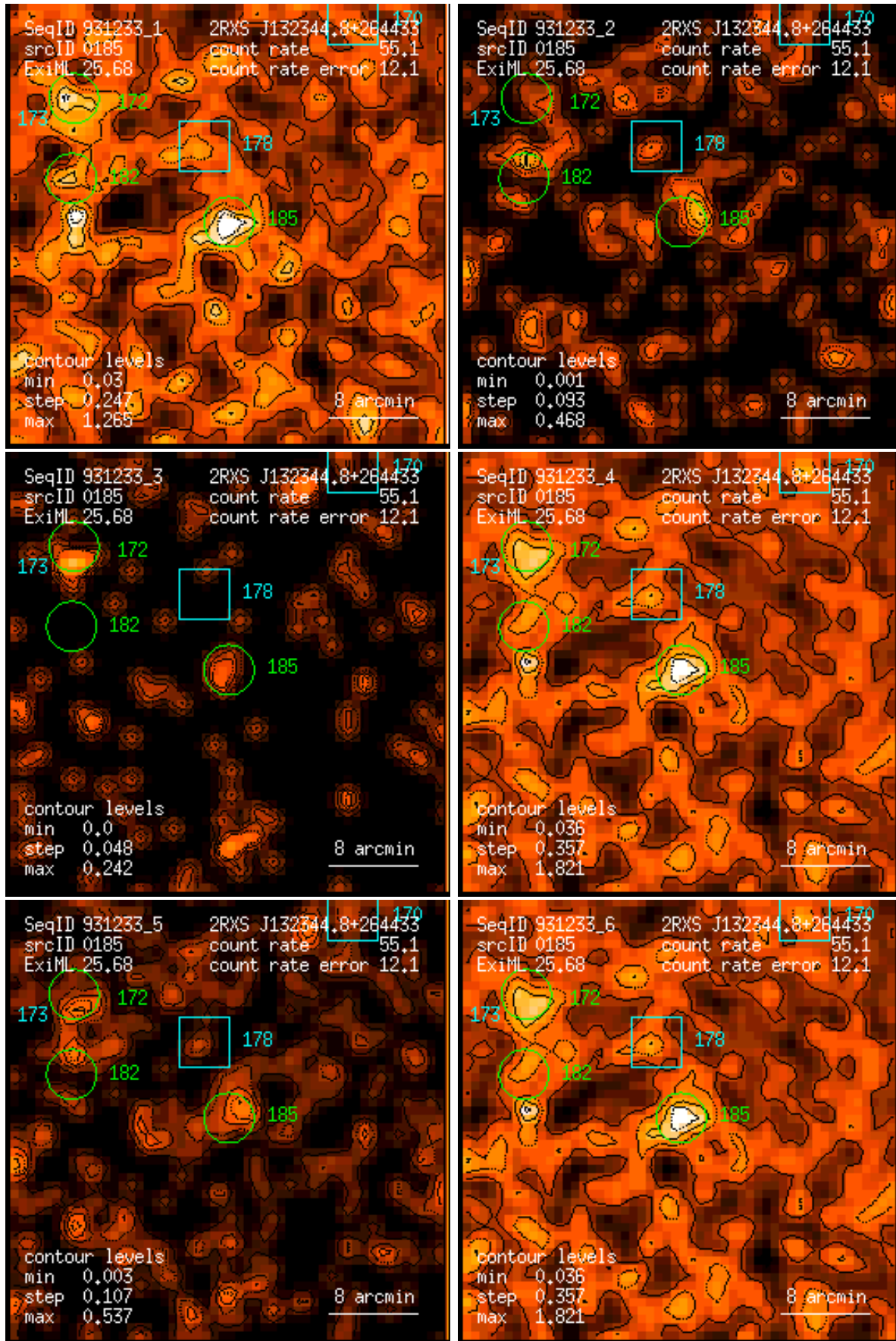
Figure 185: RASS 931233: detection 0185: band rate images, Gaussian filter: (1) PSPC channels 11 – 41, (2) 52 – 90, (3) 91 – 201, (4) 11 – 235, (5) 52 – 201, (6) 11 – 201. Broad band rates in counts/ks. Band rate contour levels in counts/ks/arcmin 2 .
