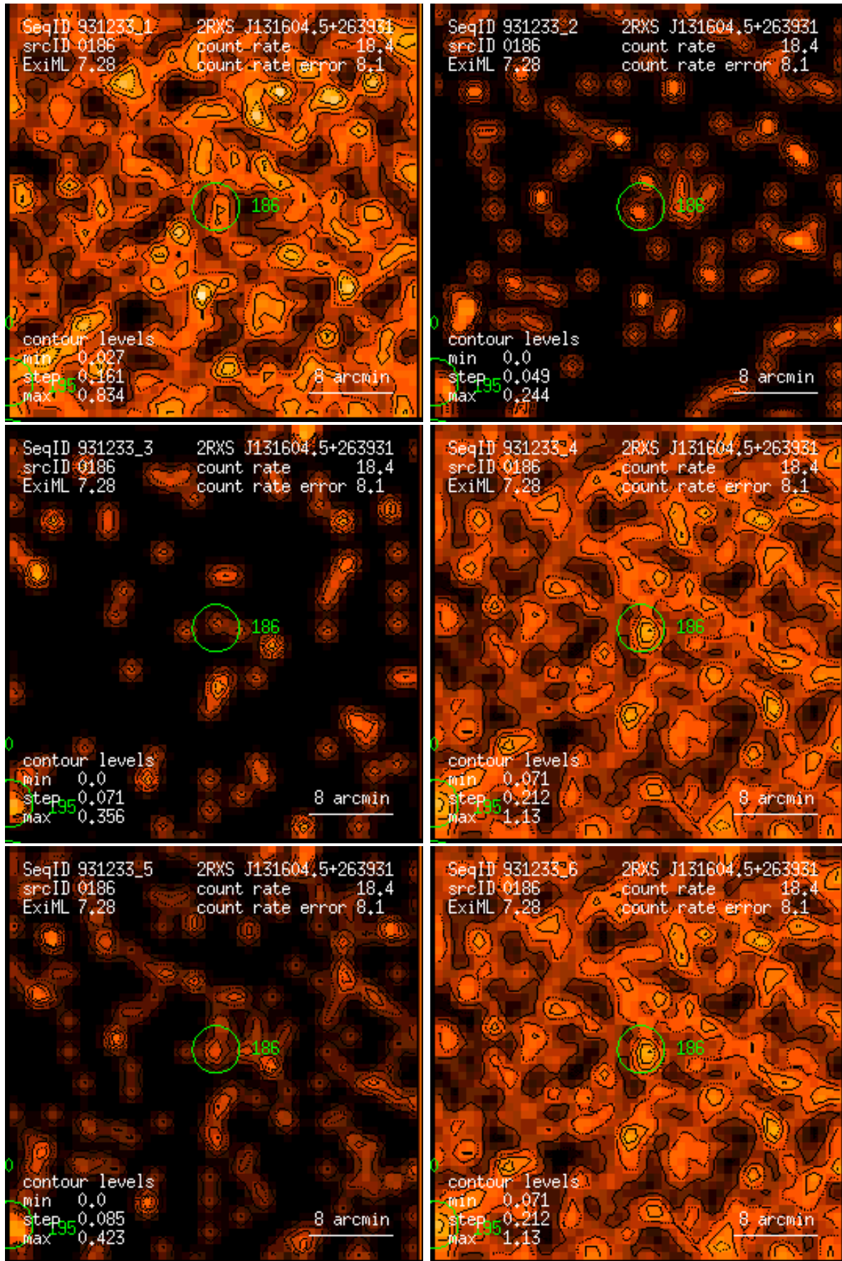
Figure 186: RASS 931233: detection 0186: band rate images, Gaussian filter: (1) PSPC channels 11 – 41, (2) 52 – 90, (3) 91 – 201, (4) 11 – 235, (5) 52 – 201, (6) 11 – 201. Broad band rates in counts/ks. Band rate contour levels in counts/ks/arcmin 2 .
