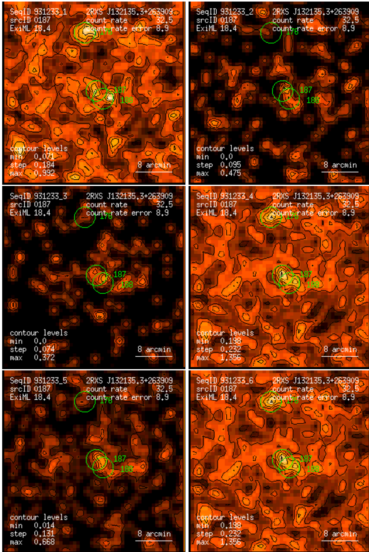
Figure 187: RASS 931233: detection 0187: band rate images, Gaussian filter: (1) PSPC channels 11 – 41, (2) 52 – 90, (3) 91 – 201, (4) 11 – 235, (5) 52 – 201, (6) 11 – 201. Broad band rates in counts/ks. Band rate contour levels in counts/ks/arcmin 2 .
