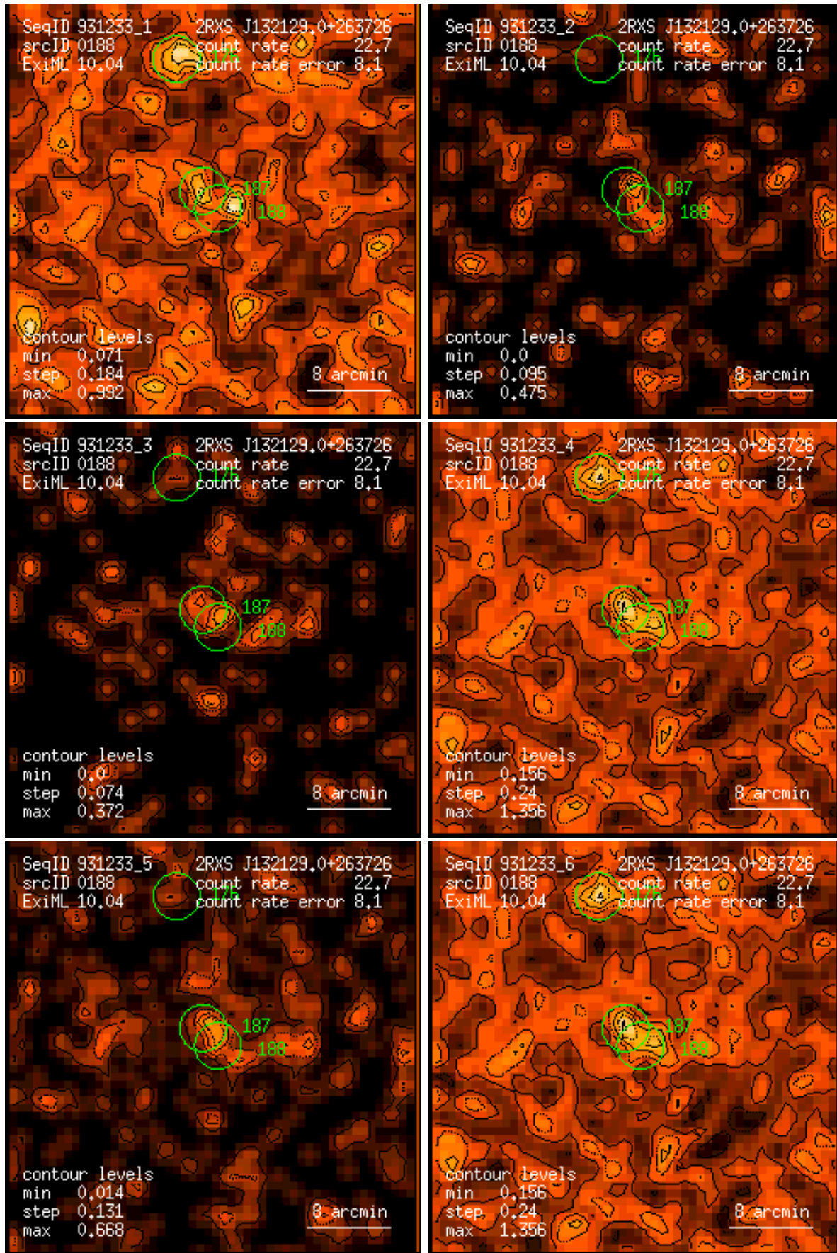
Figure 188: RASS 931233: detection 0188: band rate images, Gaussian filter: (1) PSPC channels 11 – 41, (2) 52 – 90, (3) 91 – 201, (4) 11 – 235, (5) 52 – 201, (6) 11 – 201. Broad band rates in counts/ks. Band rate contour levels in counts/ks/arcmin 2 .
