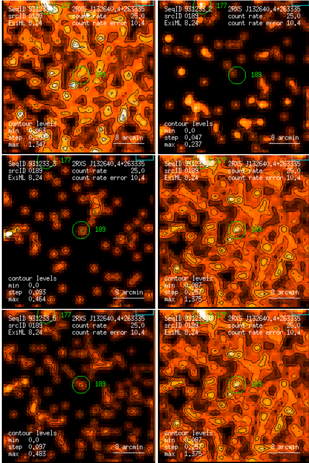
Figure 189: RASS 931233: detection 0189: band rate images, Gaussian filter: (1) PSPC channels 11 – 41, (2) 52 – 90, (3) 91 – 201, (4) 11 – 235, (5) 52 – 201, (6) 11 – 201. Broad band rates in counts/ks. Band rate contour levels in counts/ks/arcmin 2 .
