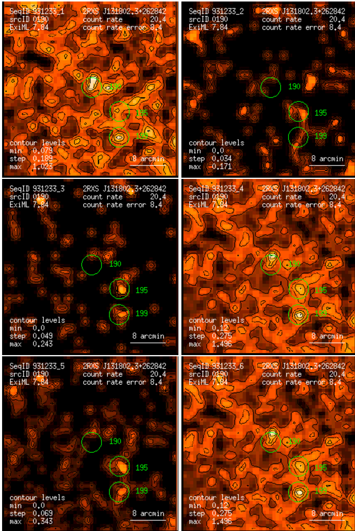
Figure 190: RASS 931233: detection 0190: band rate images, Gaussian filter: (1) PSPC channels 11 – 41, (2) 52 – 90, (3) 91 – 201, (4) 11 – 235, (5) 52 – 201, (6) 11 – 201. Broad band rates in counts/ks. Band rate contour levels in counts/ks/arcmin 2 .
