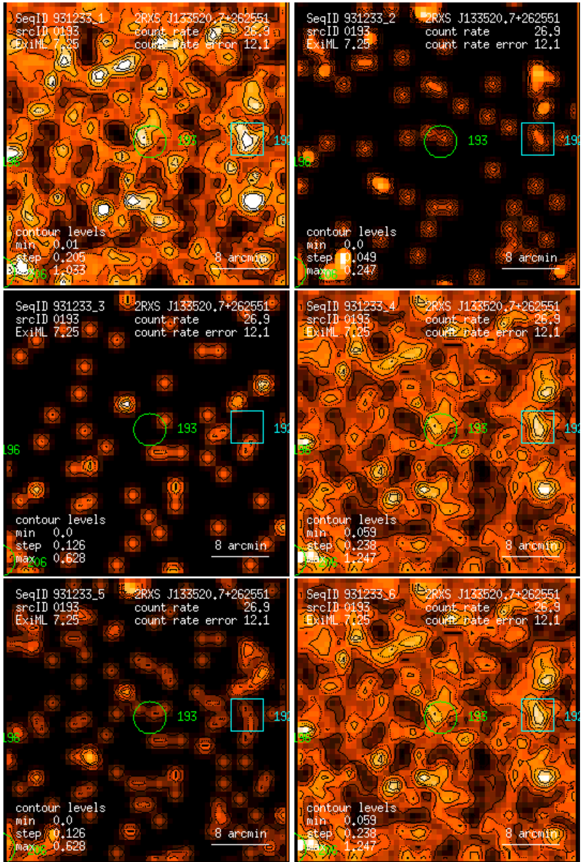
Figure 193: RASS 931233: detection 0193: band rate images, Gaussian filter: (1) PSPC channels 11 – 41, (2) 52 – 90, (3) 91 – 201, (4) 11 – 235, (5) 52 – 201, (6) 11 – 201. Broad band rates in counts/ks. Band rate contour levels in counts/ks/arcmin 2 .
