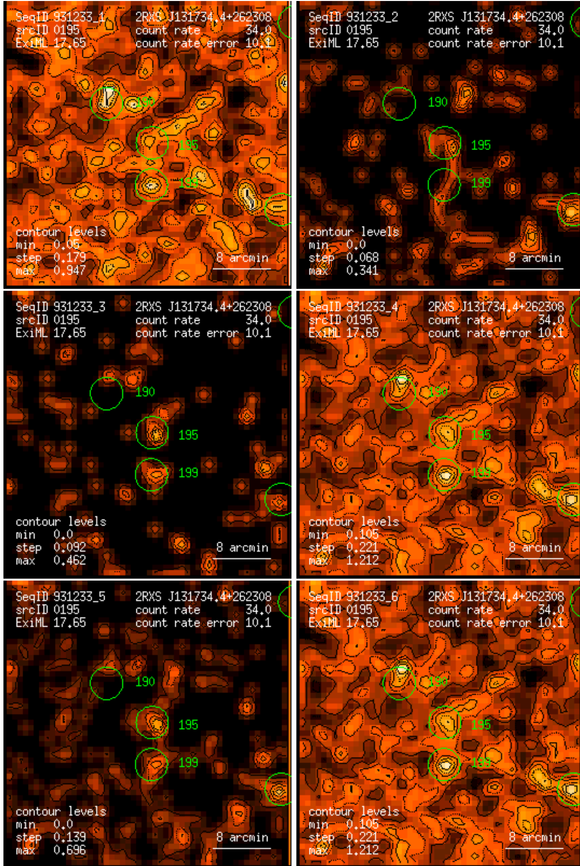
Figure 195: RASS 931233: detection 0195: band rate images, Gaussian filter: (1) PSPC channels 11 – 41, (2) 52 – 90, (3) 91 – 201, (4) 11 – 235, (5) 52 – 201, (6) 11 – 201. Broad band rates in counts/ks. Band rate contour levels in counts/ks/arcmin 2 .
