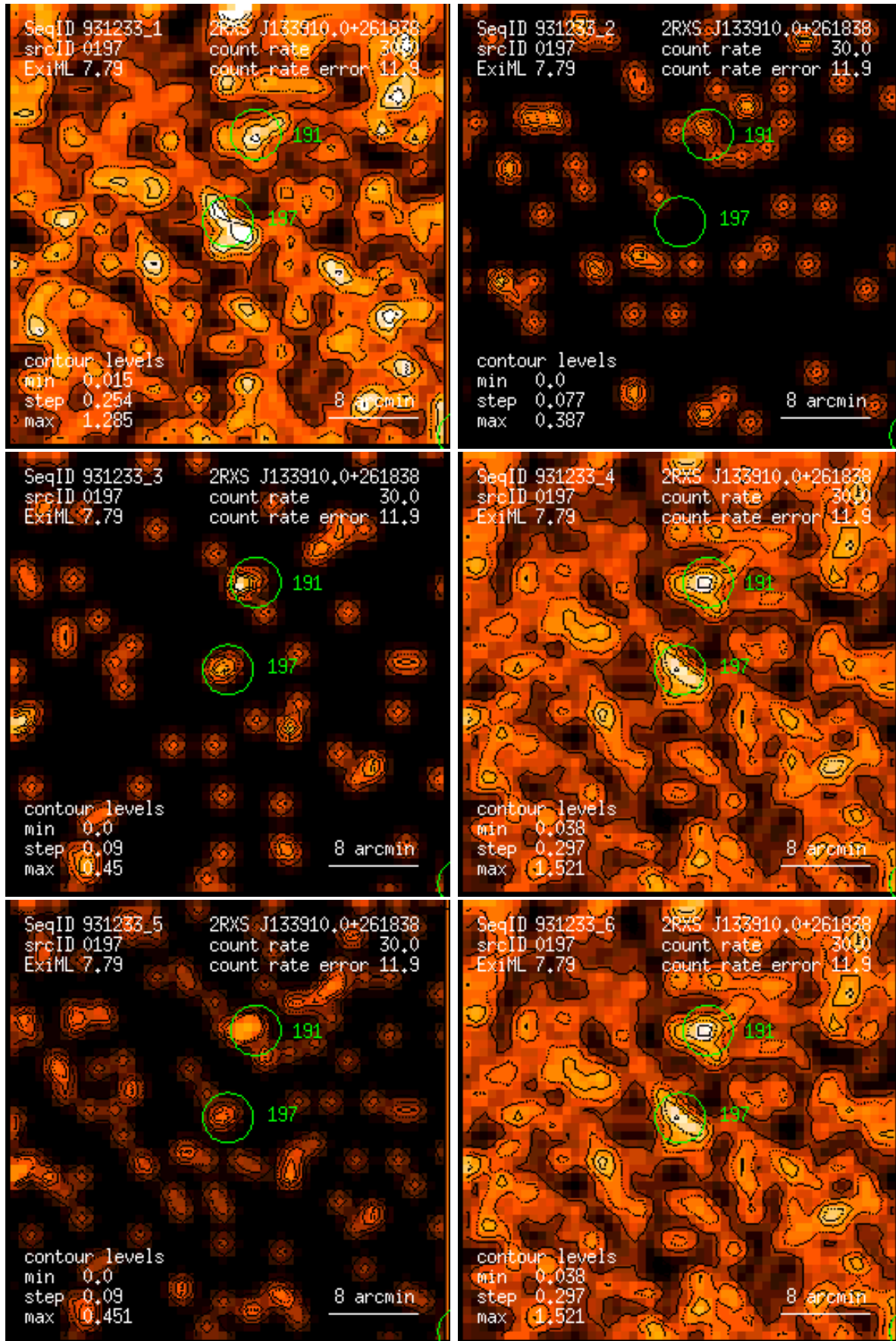
Figure 197: RASS 931233: detection 0197: band rate images, Gaussian filter: (1) PSPC channels 11 – 41, (2) 52 – 90, (3) 91 – 201, (4) 11 – 235, (5) 52 – 201, (6) 11 – 201. Broad band rates in counts/ks. Band rate contour levels in counts/ks/arcmin 2 .
