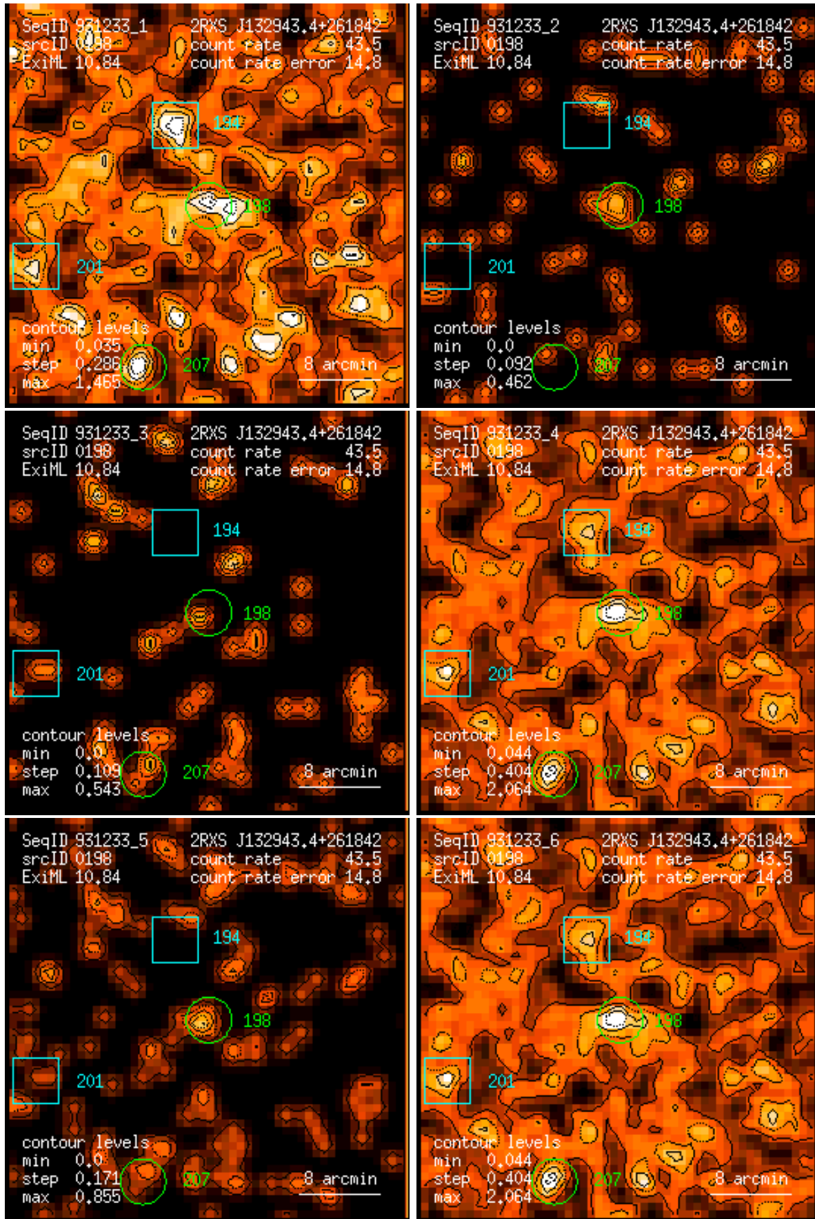
Figure 198: RASS 931233: detection 0198: band rate images, Gaussian filter: (1) PSPC channels 11 – 41, (2) 52 – 90, (3) 91 – 201, (4) 11 – 235, (5) 52 – 201, (6) 11 – 201. Broad band rates in counts/ks. Band rate contour levels in counts/ks/arcmin 2 .
