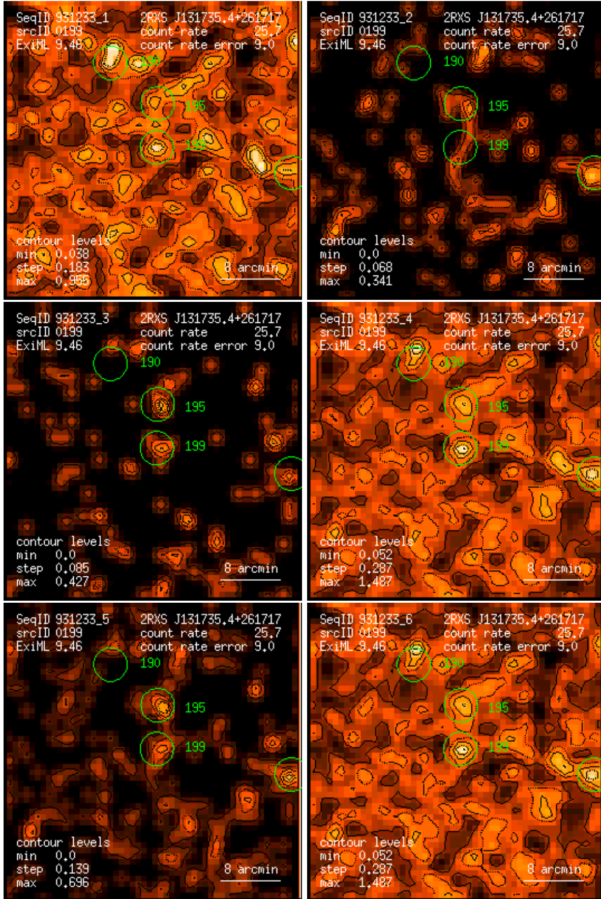
Figure 199: RASS 931233: detection 0199: band rate images, Gaussian filter: (1) PSPC channels 11 – 41, (2) 52 – 90, (3) 91 – 201, (4) 11 – 235, (5) 52 – 201, (6) 11 – 201. Broad band rates in counts/ks. Band rate contour levels in counts/ks/arcmin 2 .
