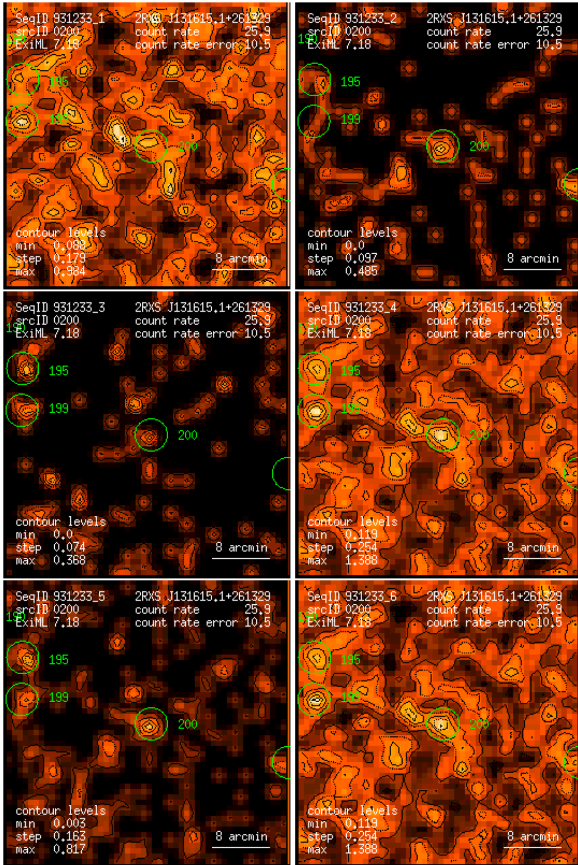
Figure 200: RASS 931233: detection 0200: band rate images, Gaussian filter: (1) PSPC channels 11 – 41, (2) 52 – 90, (3) 91 – 201, (4) 11 – 235, (5) 52 – 201, (6) 11 – 201. Broad band rates in counts/ks. Band rate contour levels in counts/ks/arcmin 2 .
