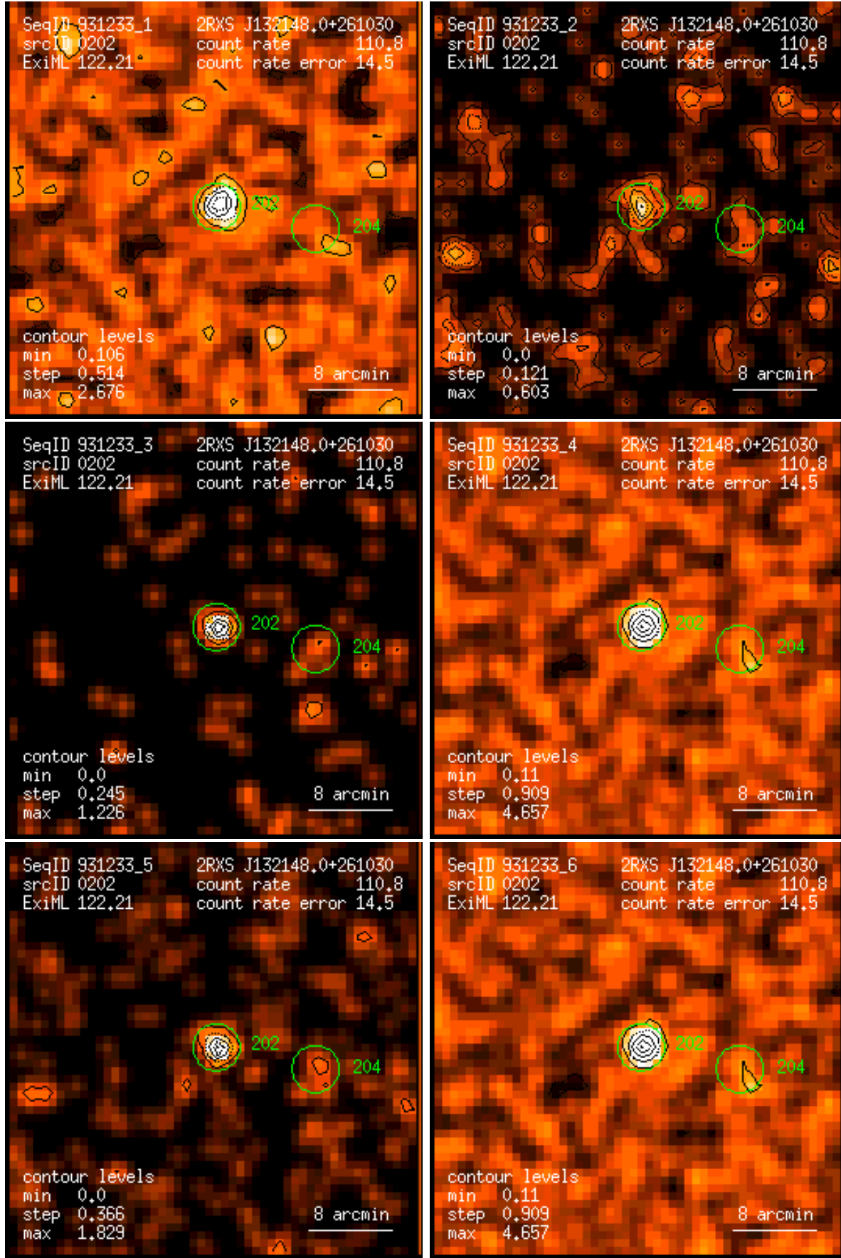
Figure 202: RASS 931233: detection 0202: band rate images, Gaussian filter: (1) PSPC channels 11 – 41, (2) 52 – 90, (3) 91 – 201, (4) 11 – 235, (5) 52 – 201, (6) 11 – 201. Broad band rates in counts/ks. Band rate contour levels in counts/ks/arcmin 2 .
