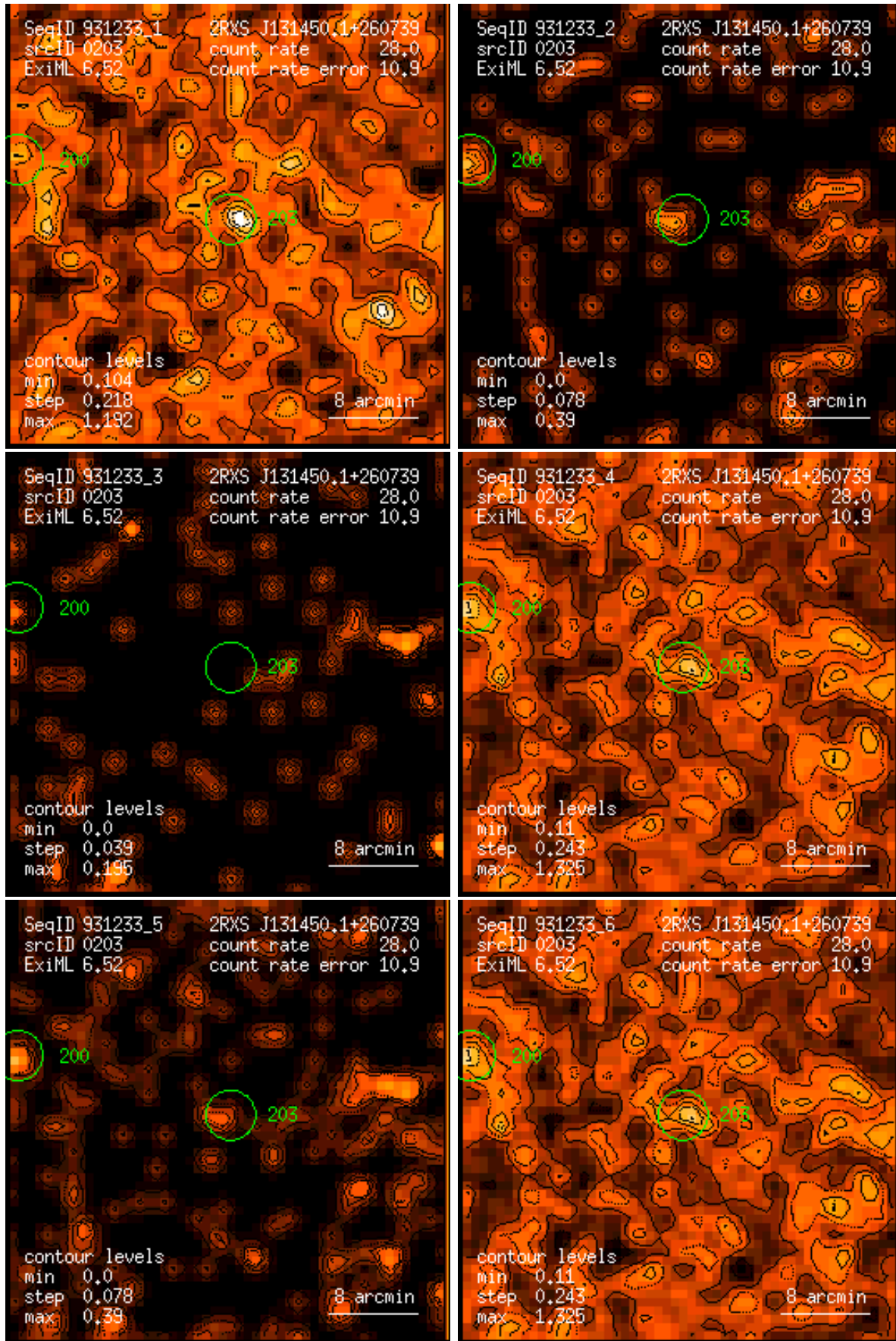
Figure 203: RASS 931233: detection 0203: band rate images, Gaussian filter: (1) PSPC channels 11 – 41, (2) 52 – 90, (3) 91 – 201, (4) 11 – 235, (5) 52 – 201, (6) 11 – 201. Broad band rates in counts/ks. Band rate contour levels in counts/ks/arcmin 2 .
