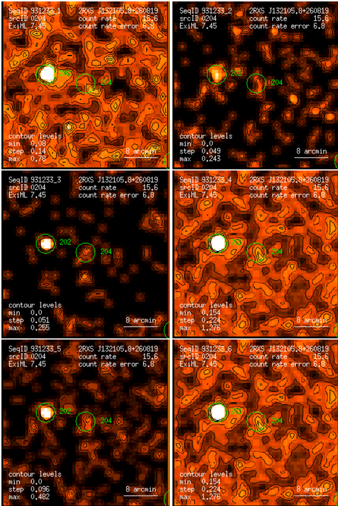
Figure 204: RASS 931233: detection 0204: band rate images, Gaussian filter: (1) PSPC channels 11 – 41, (2) 52 – 90, (3) 91 – 201, (4) 11 – 235, (5) 52 – 201, (6) 11 – 201. Broad band rates in counts/ks. Band rate contour levels in counts/ks/arcmin 2 .
