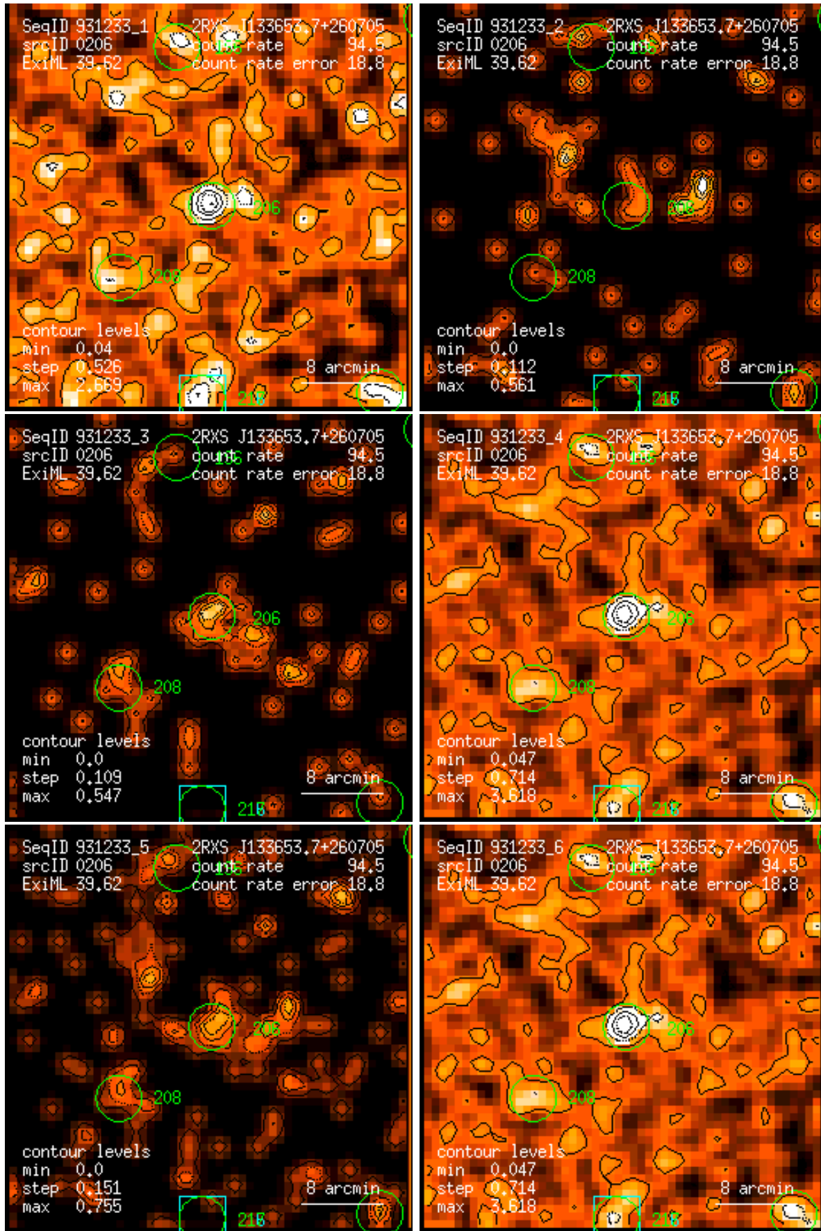
Figure 206: RASS 931233: detection 0206: band rate images, Gaussian filter: (1) PSPC channels 11 – 41, (2) 52 – 90, (3) 91 – 201, (4) 11 – 235, (5) 52 – 201, (6) 11 – 201. Broad band rates in counts/ks. Band rate contour levels in counts/ks/arcmin 2 .
