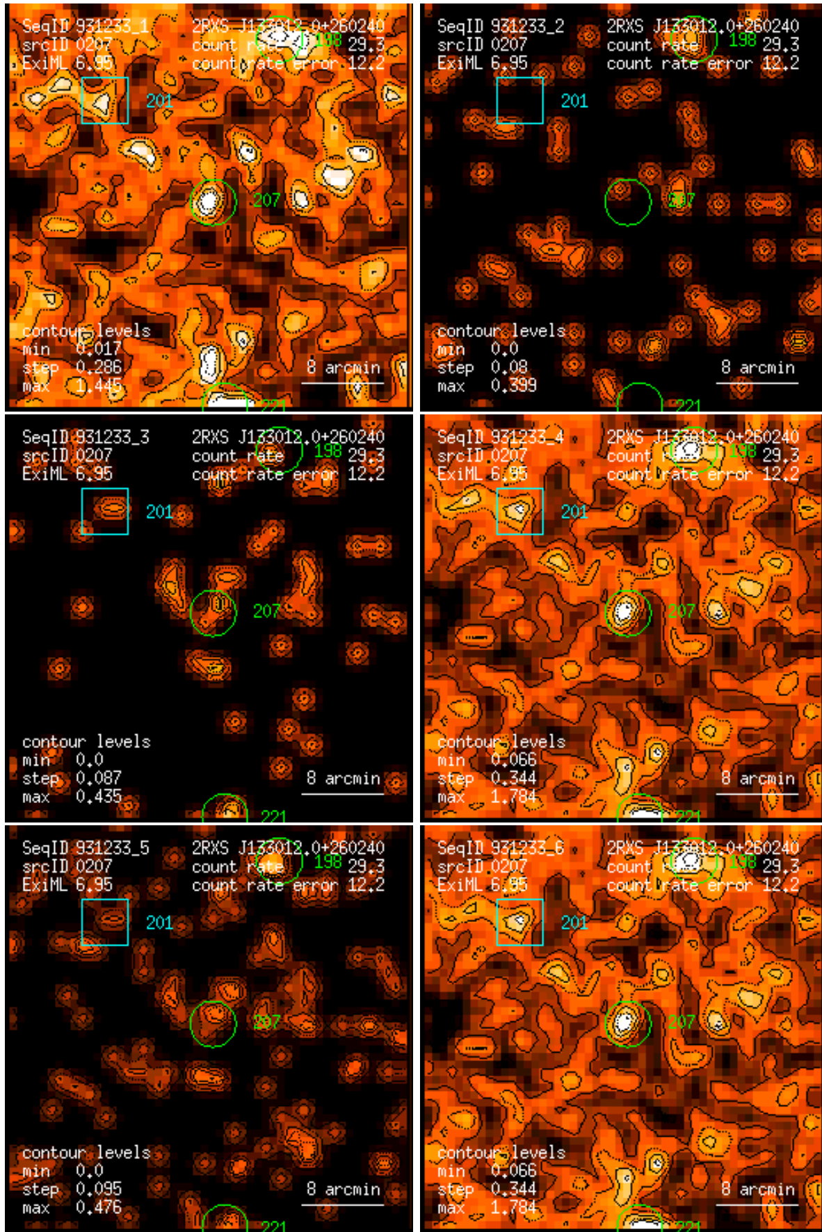
Figure 207: RASS 931233: detection 0207: band rate images, Gaussian filter: (1) PSPC channels 11 – 41, (2) 52 – 90, (3) 91 – 201, (4) 11 – 235, (5) 52 – 201, (6) 11 – 201. Broad band rates in counts/ks. Band rate contour levels in counts/ks/arcmin 2 .
