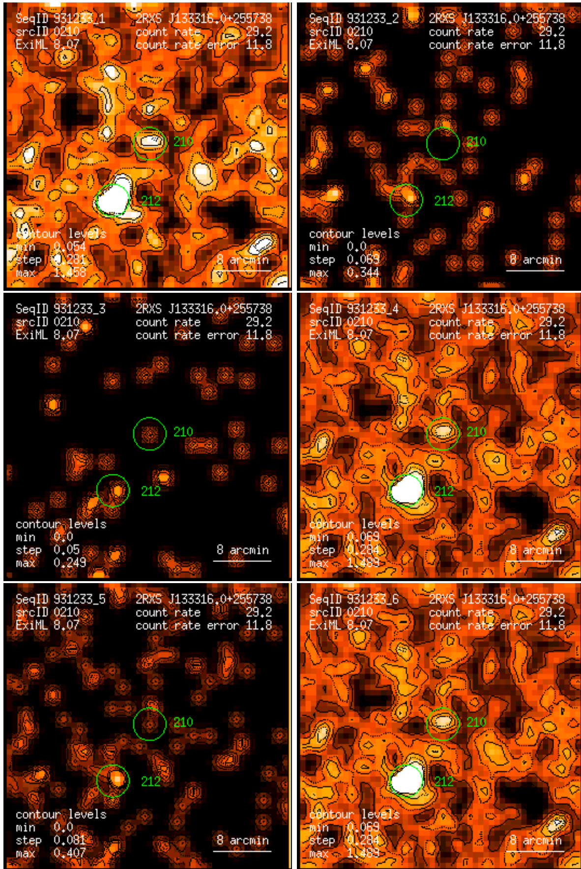
Figure 210: RASS 931233: detection 0210: band rate images, Gaussian filter: (1) PSPC channels 11 – 41, (2) 52 – 90, (3) 91 – 201, (4) 11 – 235, (5) 52 – 201, (6) 11 – 201. Broad band rates in counts/ks. Band rate contour levels in counts/ks/arcmin 2 .
