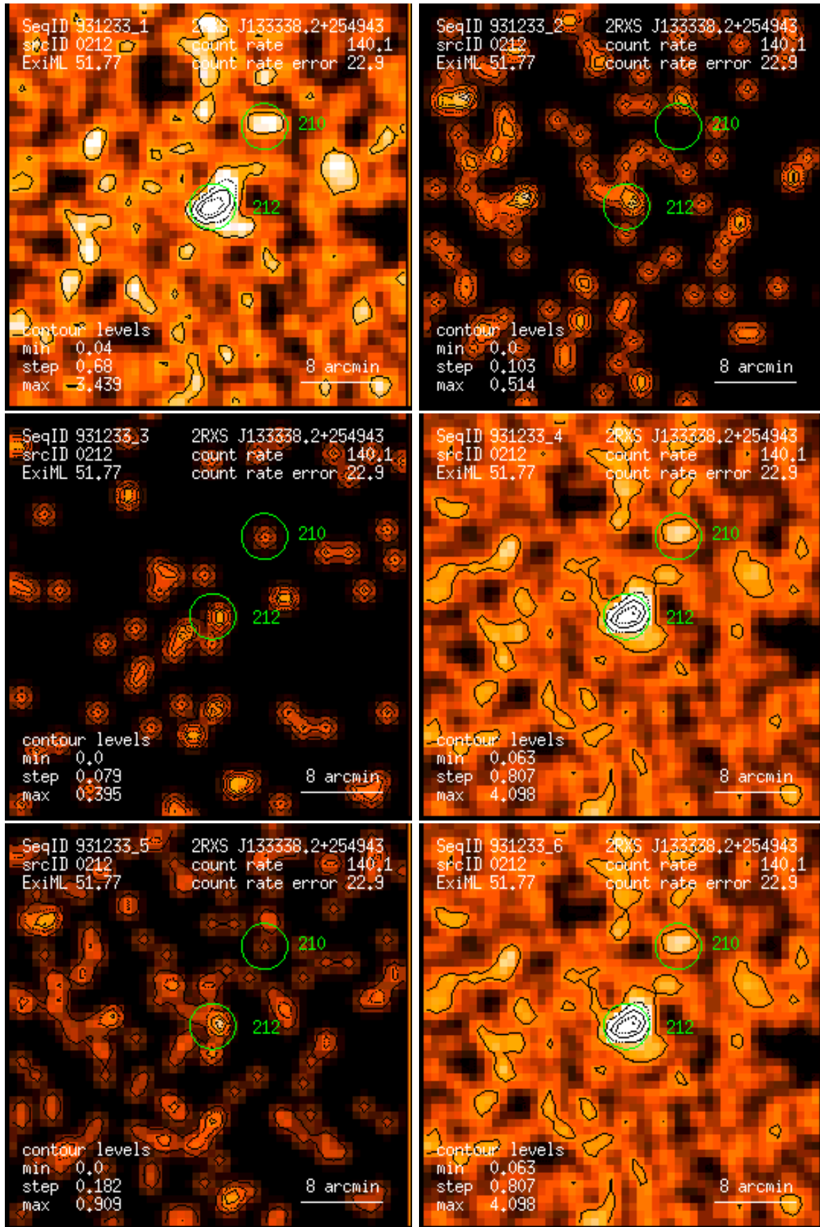
Figure 212: RASS 931233: detection 0212: band rate images, Gaussian filter: (1) PSPC channels 11 – 41, (2) 52 – 90, (3) 91 – 201, (4) 11 – 235, (5) 52 – 201, (6) 11 – 201. Broad band rates in counts/ks. Band rate contour levels in counts/ks/arcmin 2 .
