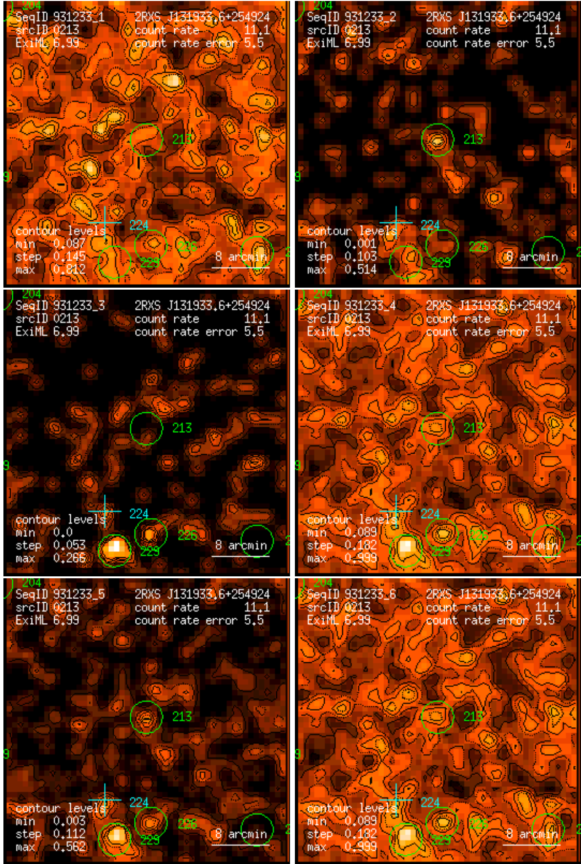
Figure 213: RASS 931233: detection 0213: band rate images, Gaussian filter: (1) PSPC channels 11 – 41, (2) 52 – 90, (3) 91 – 201, (4) 11 – 235, (5) 52 – 201, (6) 11 – 201. Broad band rates in counts/ks. Band rate contour levels in counts/ks/arcmin 2 .
