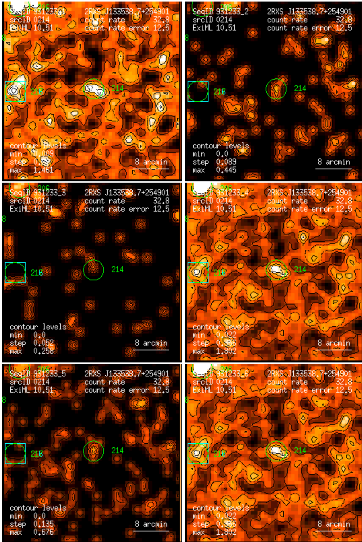
Figure 214: RASS 931233: detection 0214: band rate images, Gaussian filter: (1) PSPC channels 11 – 41, (2) 52 – 90, (3) 91 – 201, (4) 11 – 235, (5) 52 – 201, (6) 11 – 201. Broad band rates in counts/ks. Band rate contour levels in counts/ks/arcmin 2 .
