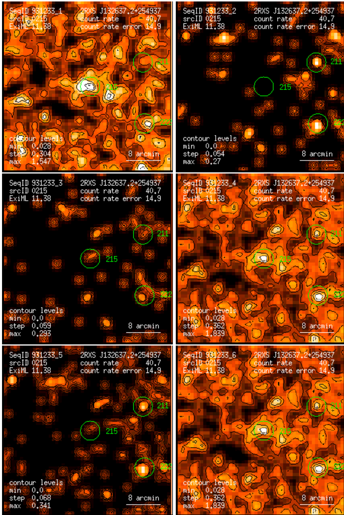
Figure 215: RASS 931233: detection 0215: band rate images, Gaussian filter: (1) PSPC channels 11 – 41, (2) 52 – 90, (3) 91 – 201, (4) 11 – 235, (5) 52 – 201, (6) 11 – 201. Broad band rates in counts/ks. Band rate contour levels in counts/ks/arcmin 2 .
