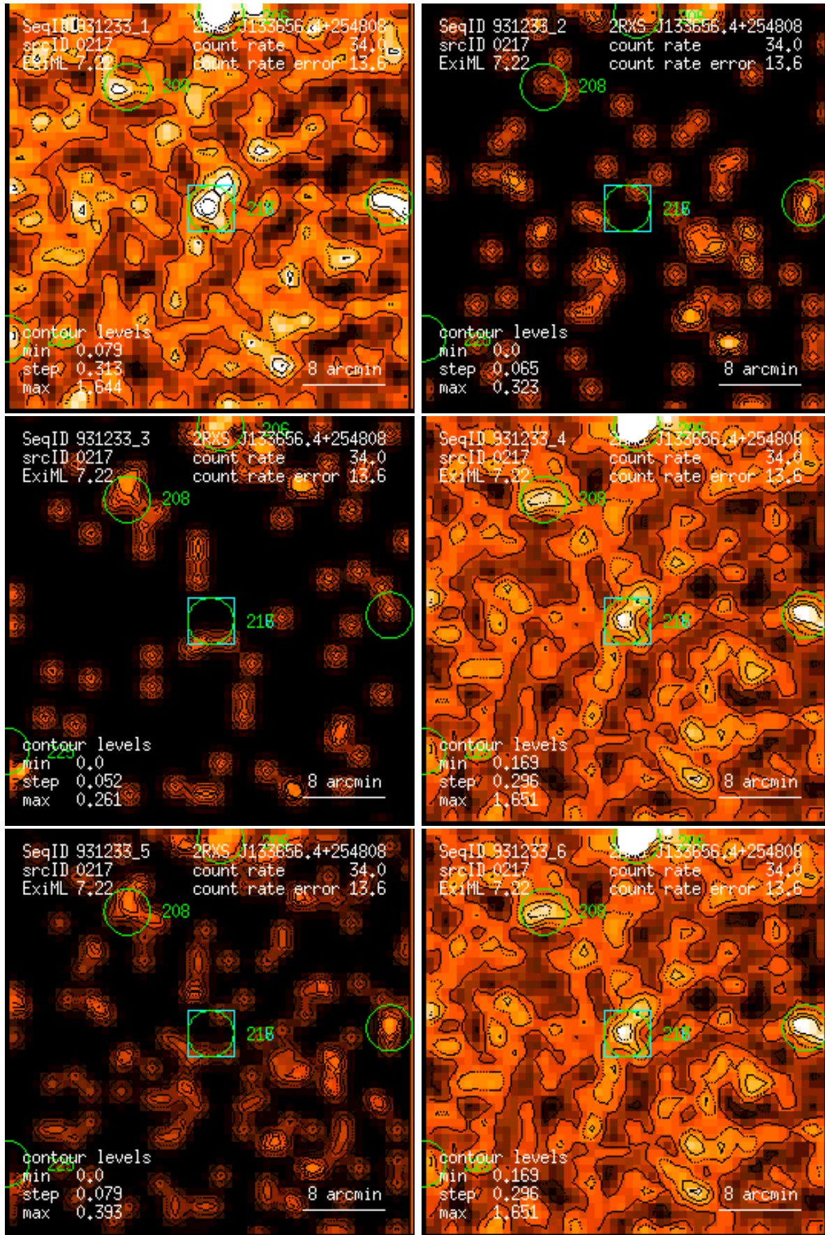
Figure 217: RASS 931233: detection 0217: band rate images, Gaussian filter: (1) PSPC channels 11 – 41, (2) 52 – 90, (3) 91 – 201, (4) 11 – 235, (5) 52 – 201, (6) 11 – 201. Broad band rates in counts/ks. Band rate contour levels in counts/ks/arcmin 2 .
