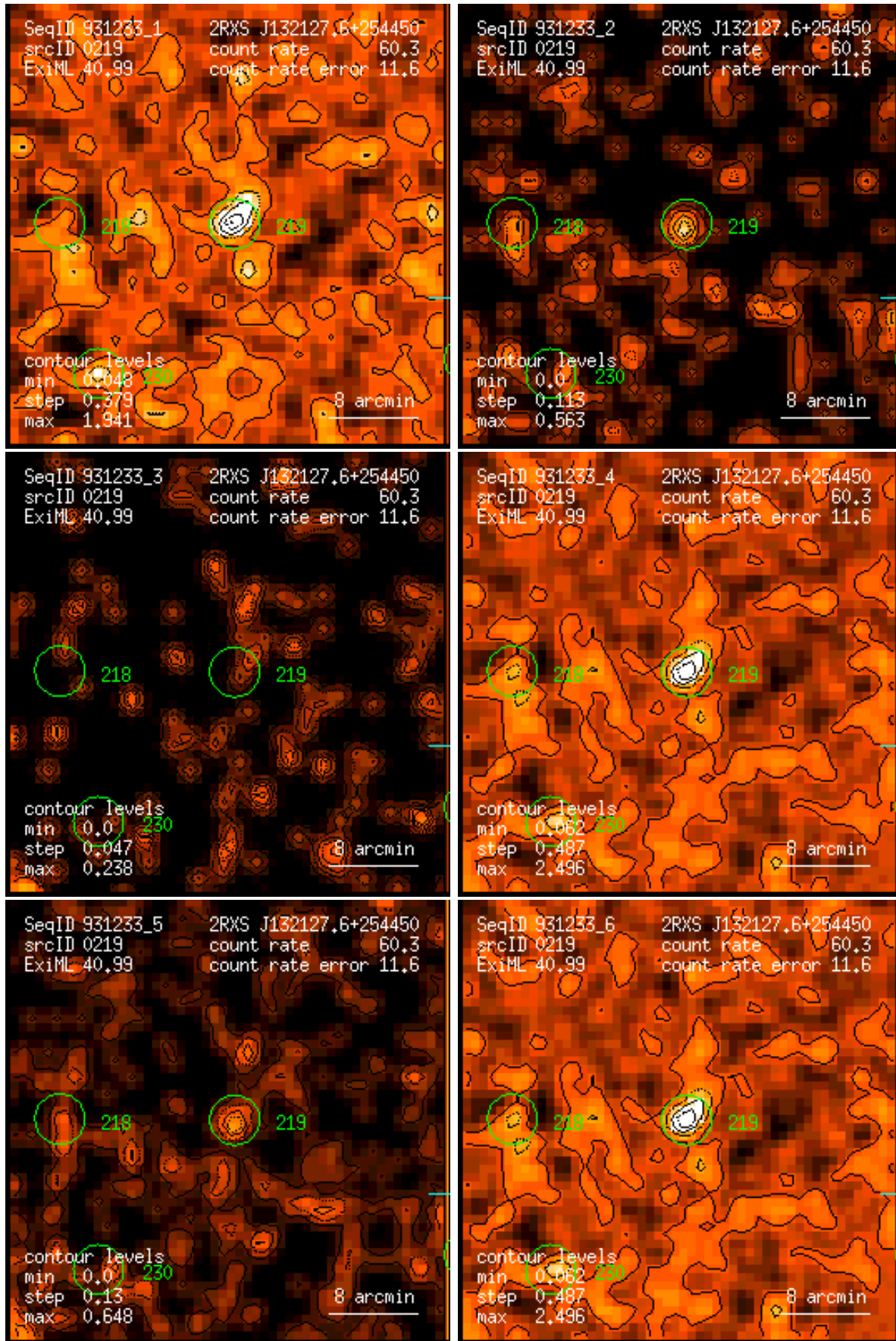
Figure 219: RASS 931233: detection 0219: band rate images, Gaussian filter: (1) PSPC channels 11 – 41, (2) 52 – 90, (3) 91 – 201, (4) 11 – 235, (5) 52 – 201, (6) 11 – 201. Broad band rates in counts/ks. Band rate contour levels in counts/ks/arcmin 2 .
