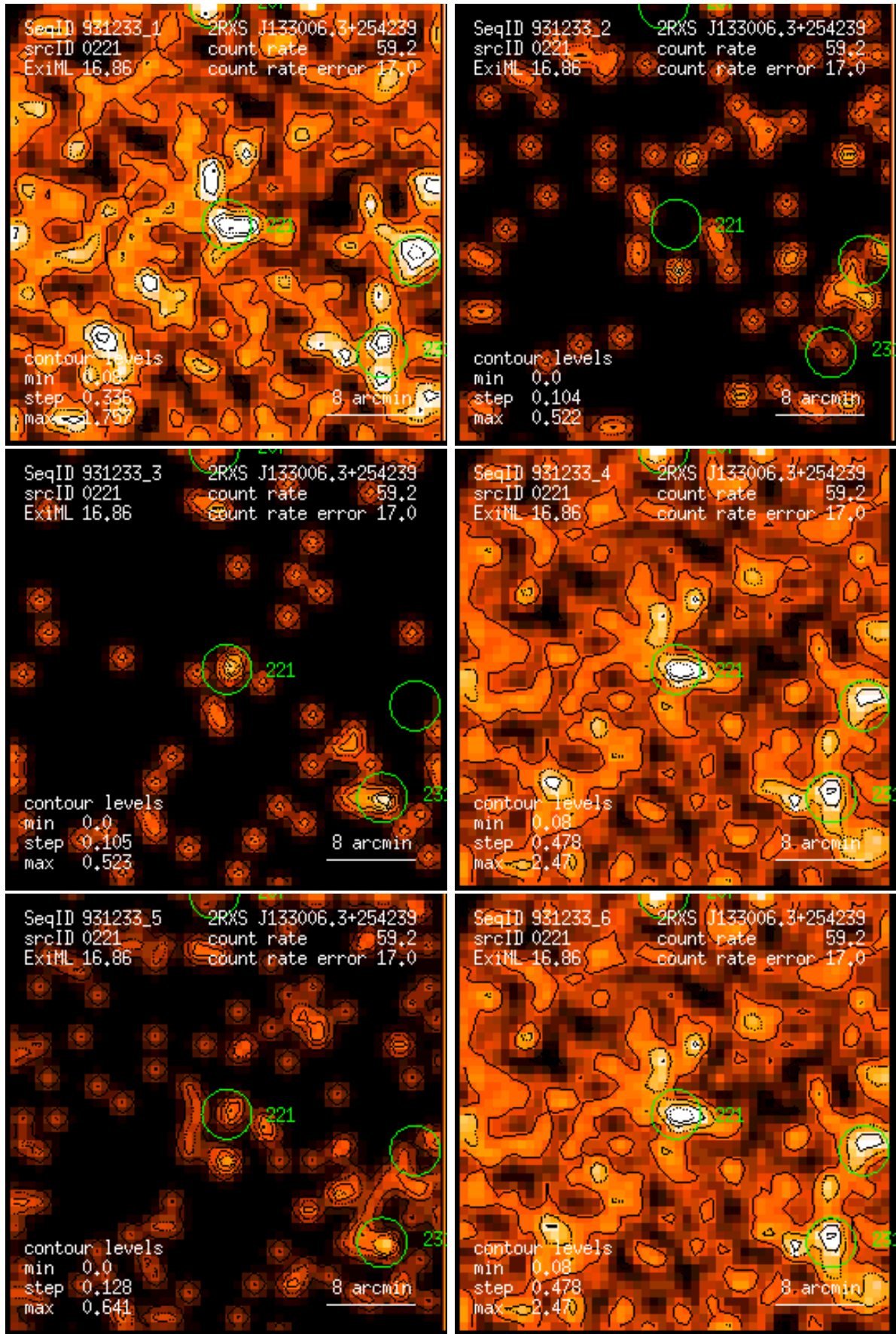
Figure 221: RASS 931233: detection 0221: band rate images, Gaussian filter: (1) PSPC channels 11 – 41, (2) 52 – 90, (3) 91 – 201, (4) 11 – 235, (5) 52 – 201, (6) 11 – 201. Broad band rates in counts/ks. Band rate contour levels in counts/ks/arcmin 2 .
