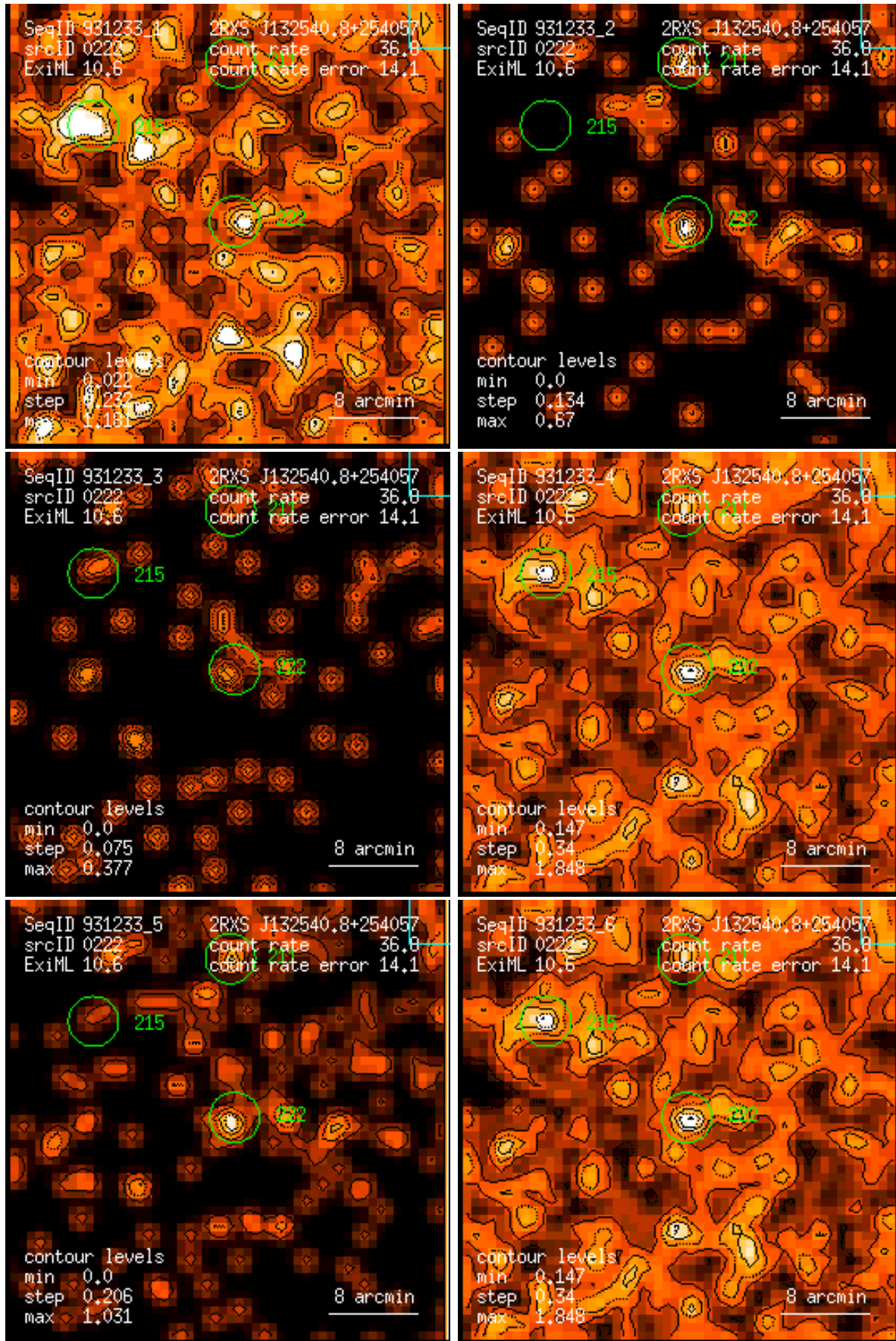
Figure 222: RASS 931233: detection 0222: band rate images, Gaussian filter: (1) PSPC channels 11 – 41, (2) 52 – 90, (3) 91 – 201, (4) 11 – 235, (5) 52 – 201, (6) 11 – 201. Broad band rates in counts/ks. Band rate contour levels in counts/ks/arcmin 2 .
