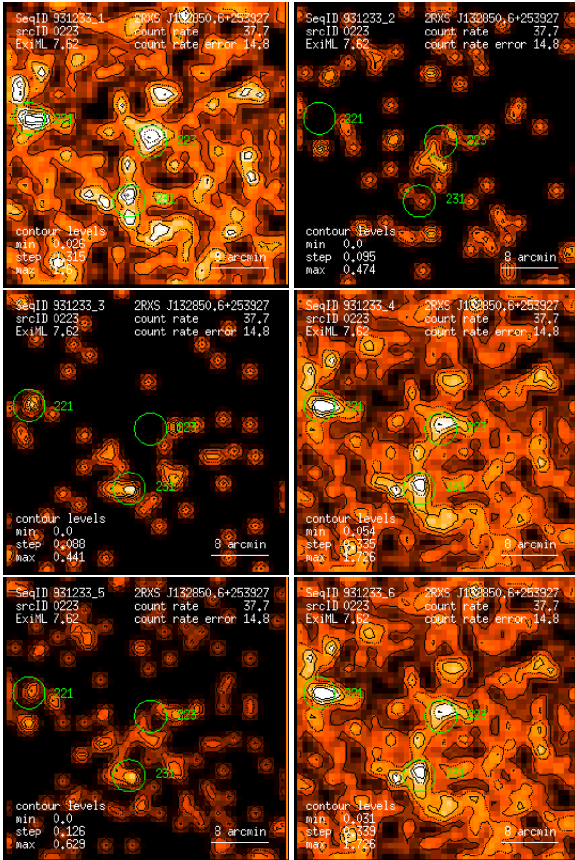
Figure 223: RASS 931233: detection 0223: band rate images, Gaussian filter: (1) PSPC channels 11 – 41, (2) 52 – 90, (3) 91 – 201, (4) 11 – 235, (5) 52 – 201, (6) 11 – 201. Broad band rates in counts/ks. Band rate contour levels in counts/ks/arcmin 2 .
