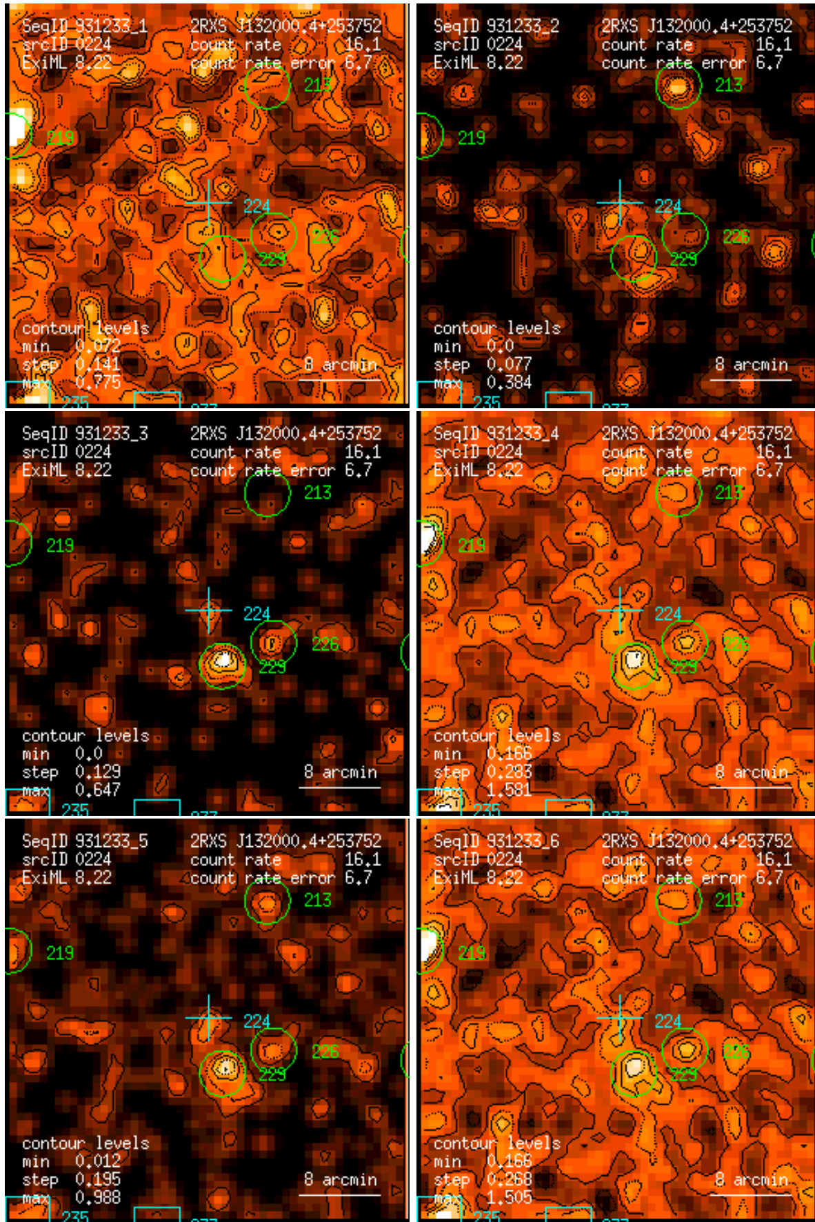
Figure 224: RASS 931233: detection 0224: band rate images, Gaussian filter: (1) PSPC channels 11 – 41, (2) 52 – 90, (3) 91 – 201, (4) 11 – 235, (5) 52 – 201, (6) 11 – 201. Broad band rates in counts/ks. Band rate contour levels in counts/ks/arcmin 2 .
