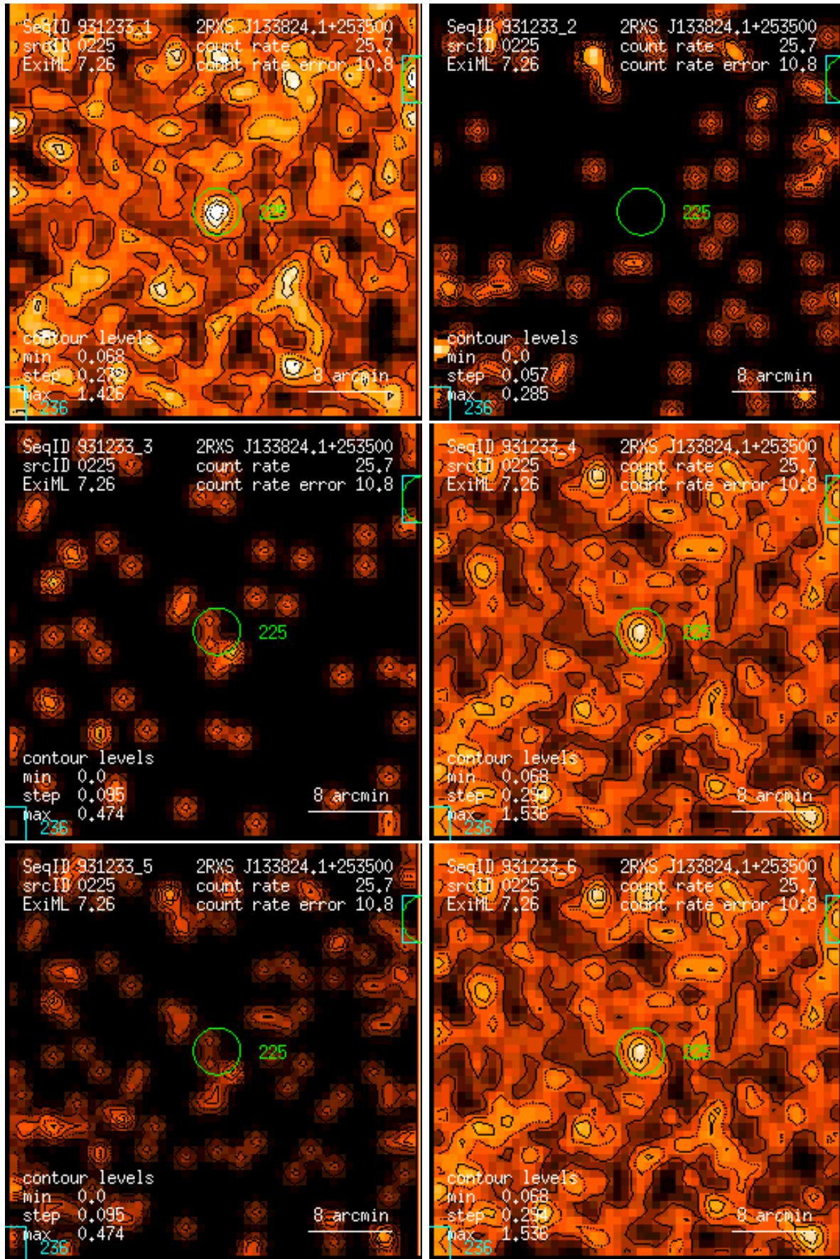
Figure 225: RASS 931233: detection 0225: band rate images, Gaussian filter: (1) PSPC channels 11 – 41, (2) 52 – 90, (3) 91 – 201, (4) 11 – 235, (5) 52 – 201, (6) 11 – 201. Broad band rates in counts/ks. Band rate contour levels in counts/ks/arcmin 2 .
