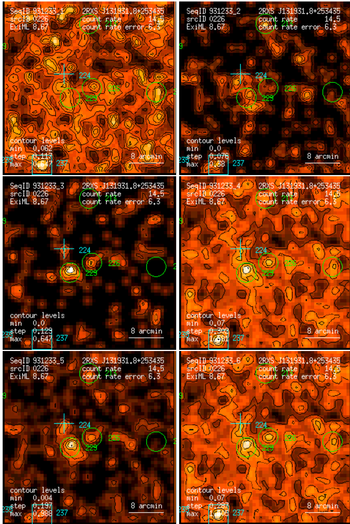
Figure 226: RASS 931233: detection 0226: band rate images, Gaussian filter: (1) PSPC channels 11 – 41, (2) 52 – 90, (3) 91 – 201, (4) 11 – 235, (5) 52 – 201, (6) 11 – 201. Broad band rates in counts/ks. Band rate contour levels in counts/ks/arcmin 2 .
