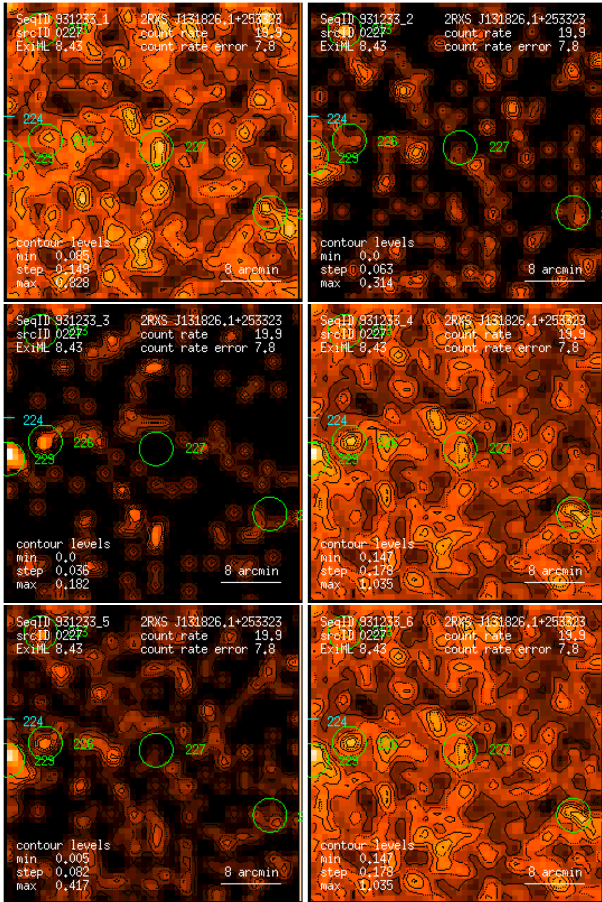
Figure 227: RASS 931233: detection 0227: band rate images, Gaussian filter: (1) PSPC channels 11 – 41, (2) 52 – 90, (3) 91 – 201, (4) 11 – 235, (5) 52 – 201, (6) 11 – 201. Broad band rates in counts/ks. Band rate contour levels in counts/ks/arcmin 2 .
