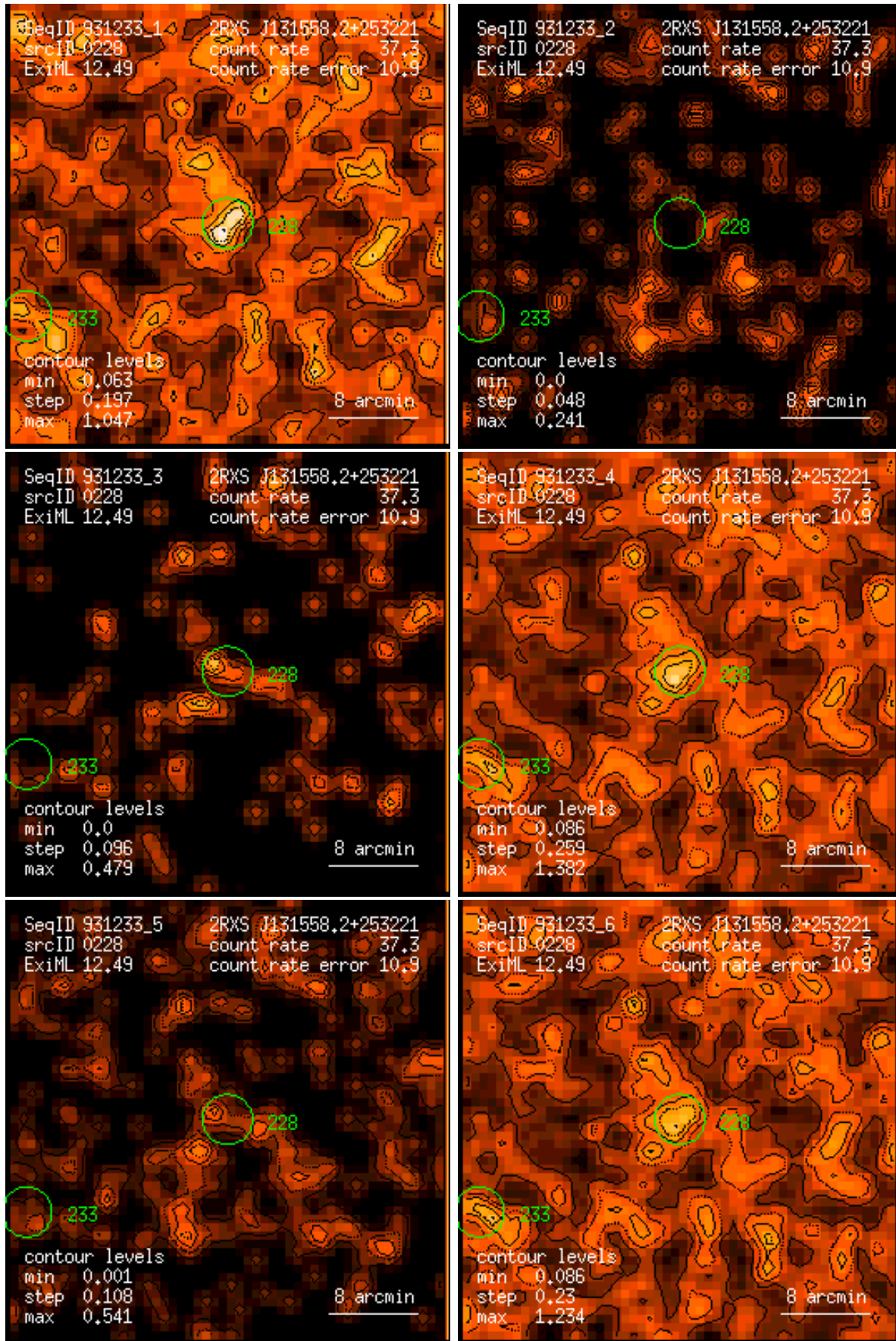
Figure 228: RASS 931233: detection 0228: band rate images, Gaussian filter: (1) PSPC channels 11 – 41, (2) 52 – 90, (3) 91 – 201, (4) 11 – 235, (5) 52 – 201, (6) 11 – 201. Broad band rates in counts/ks. Band rate contour levels in counts/ks/arcmin 2 .
