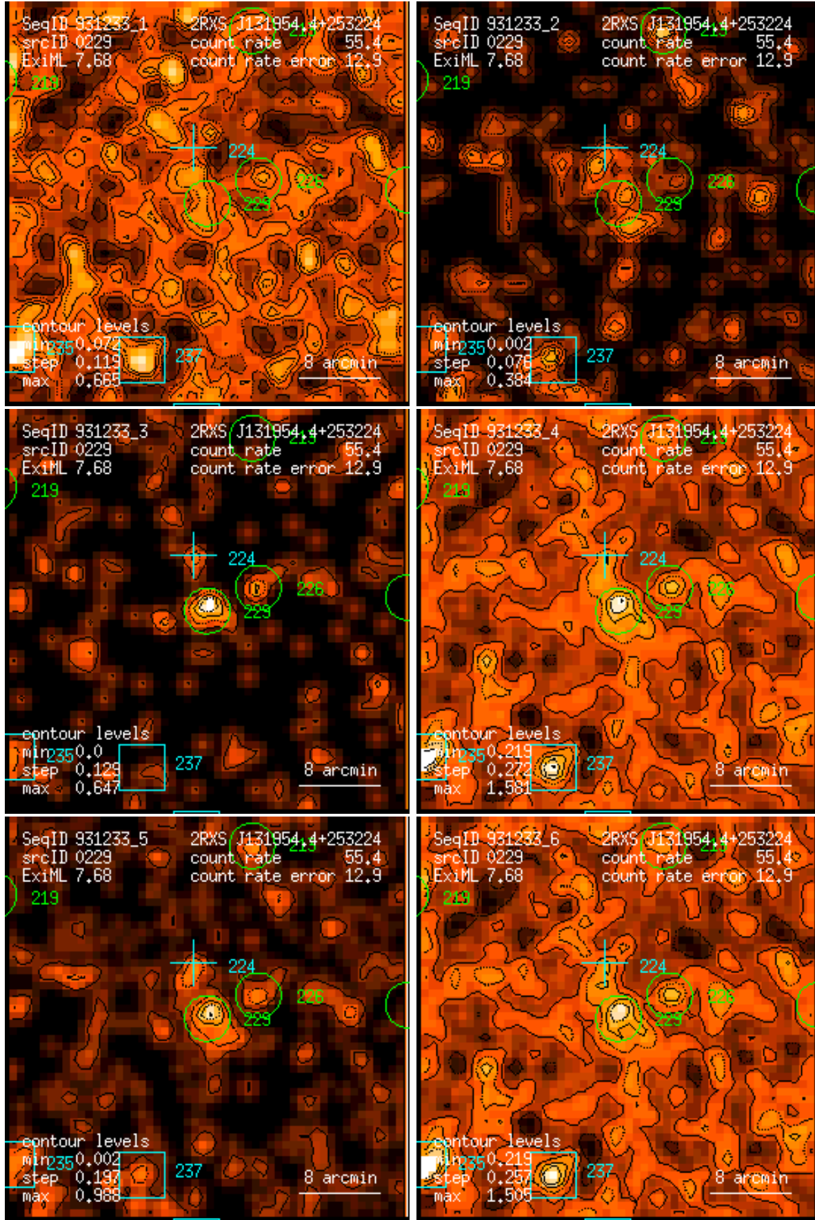
Figure 229: RASS 931233: detection 0229: band rate images, Gaussian filter: (1) PSPC channels 11 – 41, (2) 52 – 90, (3) 91 – 201, (4) 11 – 235, (5) 52 – 201, (6) 11 – 201. Broad band rates in counts/ks. Band rate contour levels in counts/ks/arcmin 2 .
