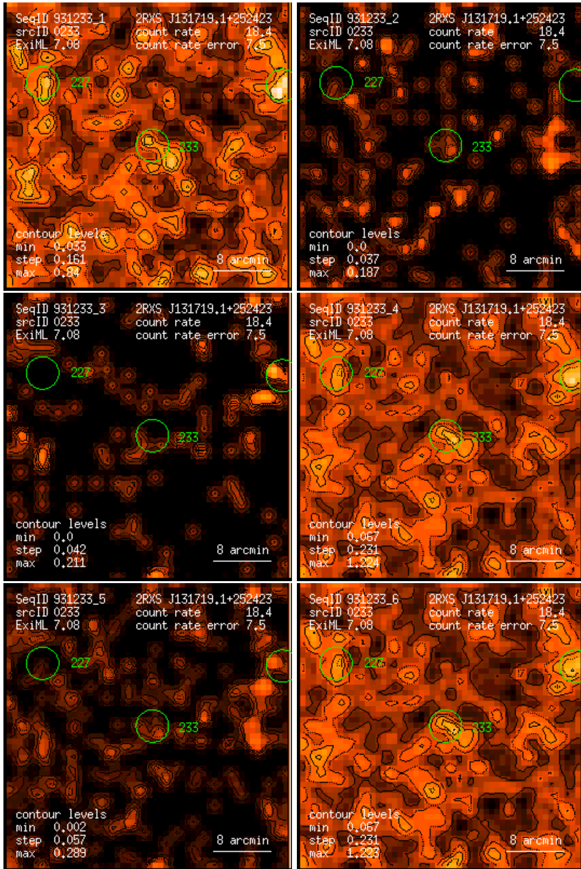
Figure 233: RASS 931233: detection 0233: band rate images, Gaussian filter: (1) PSPC channels 11 – 41, (2) 52 – 90, (3) 91 – 201, (4) 11 – 235, (5) 52 – 201, (6) 11 – 201. Broad band rates in counts/ks. Band rate contour levels in counts/ks/arcmin 2 .
