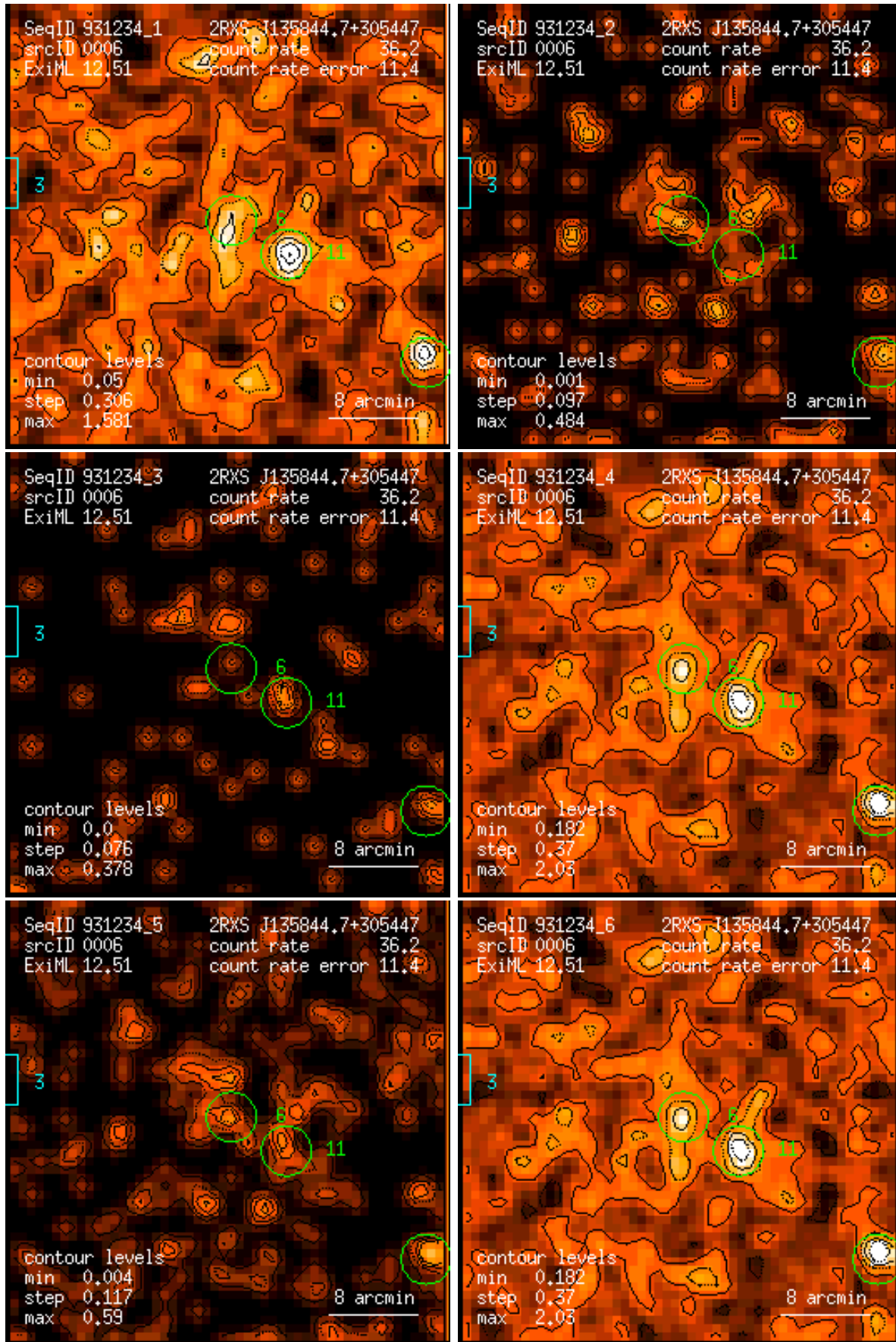
Figure 6: RASS 931234: detection 0006: band rate images, Gaussian filter: (1) PSPC channels 11 – 41, (2) 52 – 90, (3) 91 – 201, (4) 11 – 235, (5) 52 – 201, (6) 11 – 201. Broad band rates in counts/ks. Band rate contour levels in counts/ks/arcmin 2 .
