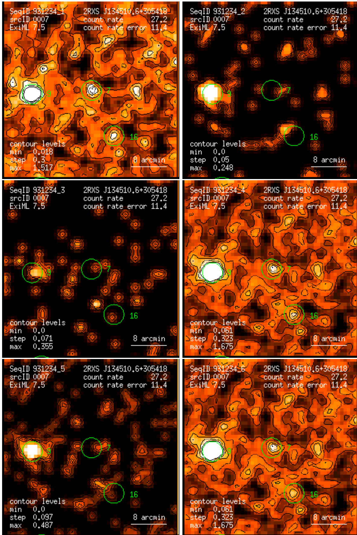
Figure 7: RASS 931234: detection 0007: band rate images, Gaussian filter: (1) PSPC channels 11 – 41, (2) 52 – 90, (3) 91 – 201, (4) 11 – 235, (5) 52 – 201, (6) 11 – 201. Broad band rates in counts/ks. Band rate contour levels in counts/ks/arcmin 2 .
