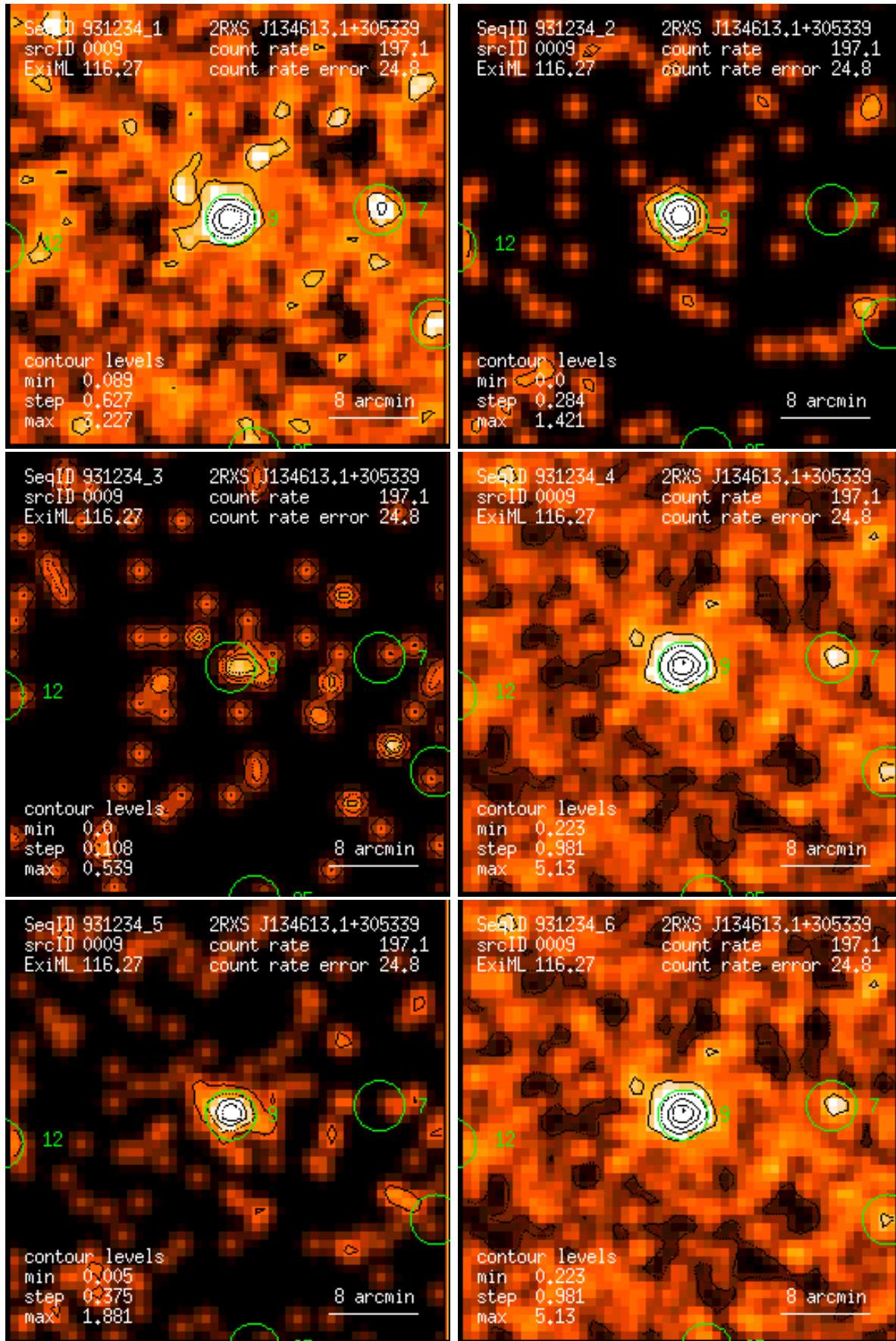
Figure 9: RASS 931234: detection 0009: band rate images, Gaussian filter: (1) PSPC channels 11 – 41, (2) 52 – 90, (3) 91 – 201, (4) 11 – 235, (5) 52 – 201, (6) 11 – 201. Broad band rates in counts/ks. Band rate contour levels in counts/ks/arcmin 2 .
