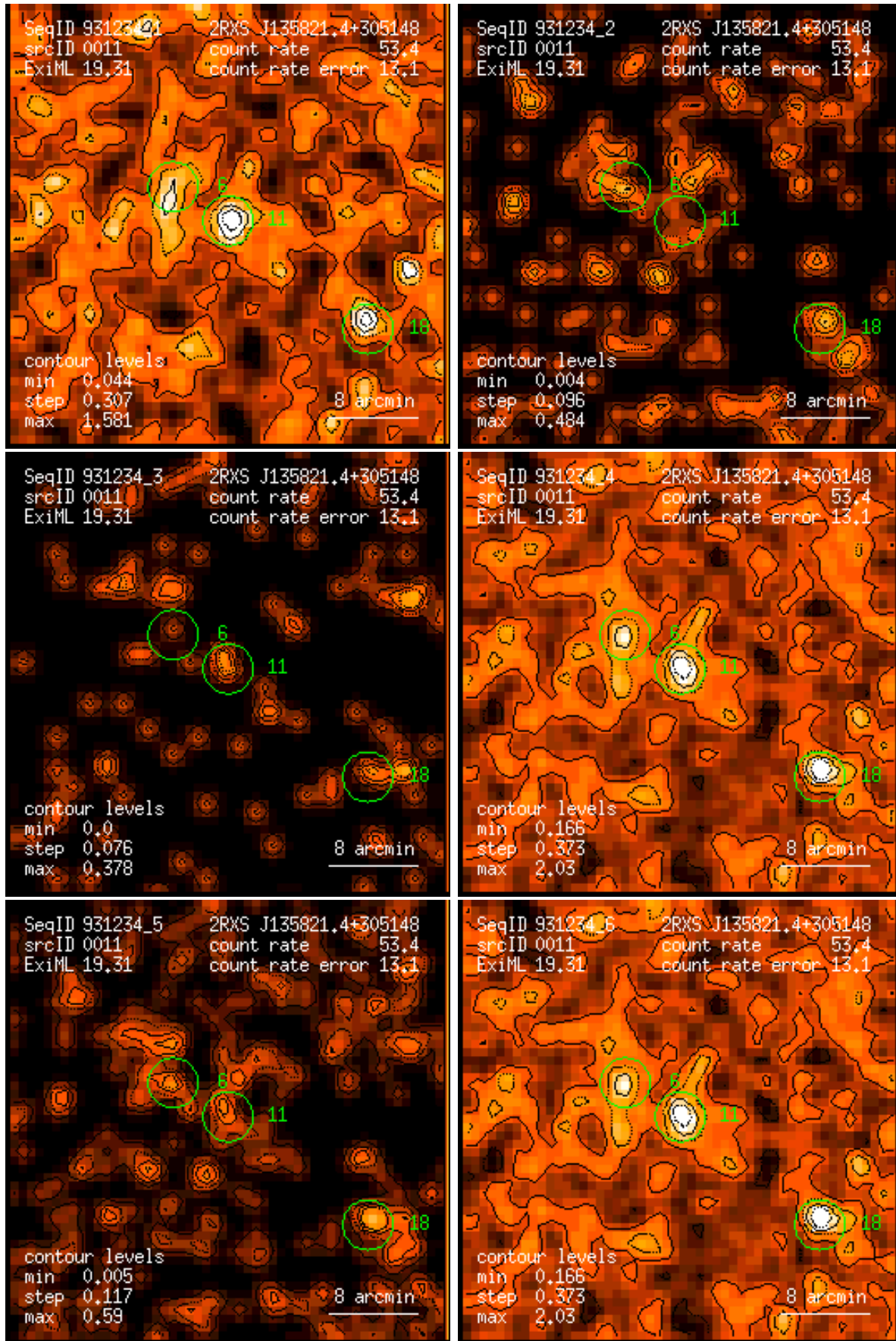
Figure 11: RASS 931234: detection 0011: band rate images, Gaussian filter: (1) PSPC channels 11 – 41, (2) 52 – 90, (3) 91 – 201, (4) 11 – 235, (5) 52 – 201, (6) 11 – 201. Broad band rates in counts/ks. Band rate contour levels in counts/ks/arcmin 2 .
