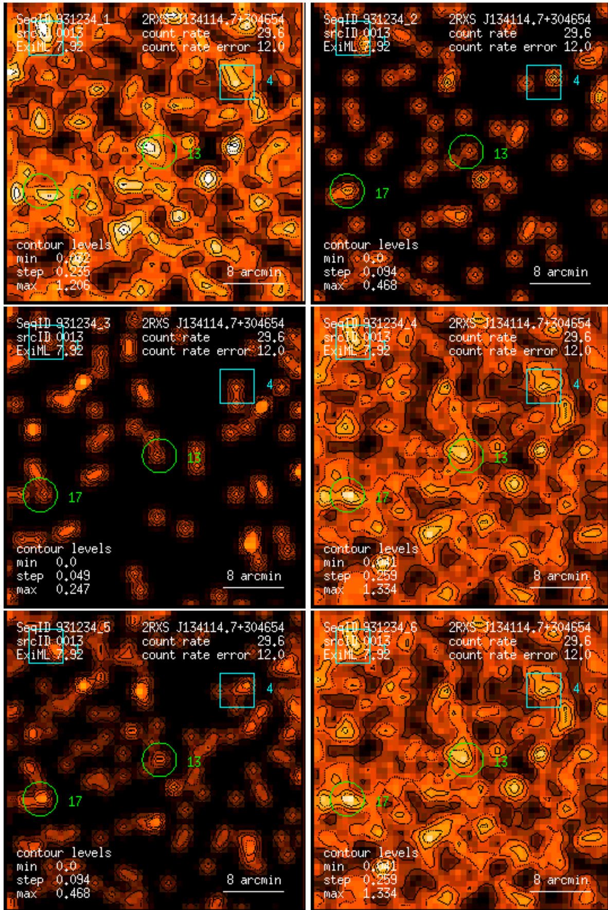
Figure 13: RASS 931234: detection 0013: band rate images, Gaussian filter: (1) PSPC channels 11 – 41, (2) 52 – 90, (3) 91 – 201, (4) 11 – 235, (5) 52 – 201, (6) 11 – 201. Broad band rates in counts/ks. Band rate contour levels in counts/ks/arcmin 2 .
