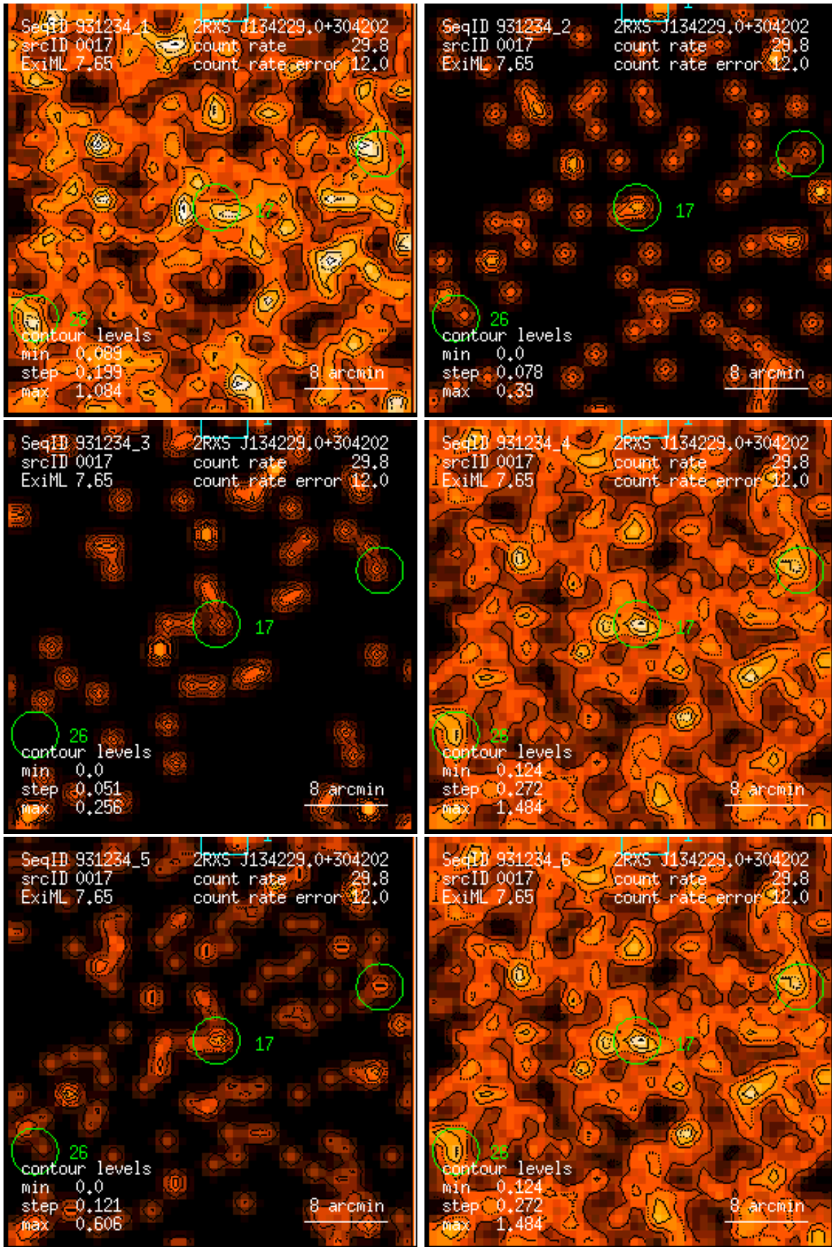
Figure 17: RASS 931234: detection 0017: band rate images, Gaussian filter: (1) PSPC channels 11 – 41, (2) 52 – 90, (3) 91 – 201, (4) 11 – 235, (5) 52 – 201, (6) 11 – 201. Broad band rates in counts/ks. Band rate contour levels in counts/ks/arcmin 2 .
